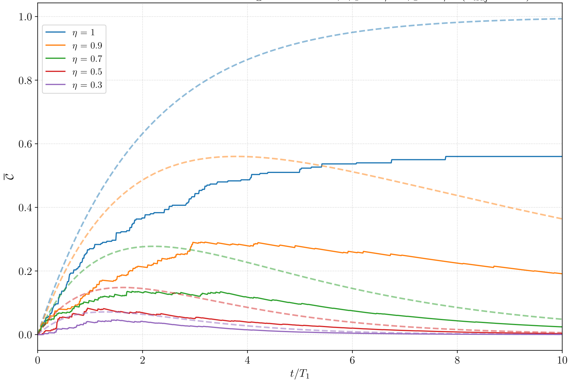
Inefficient Photodetection: Average \bar{\mathcal{C}} over time, \phi_1 = \pi/2 \phi_2 = \pi/2 ( n_{\text{traj}} = 100 )
