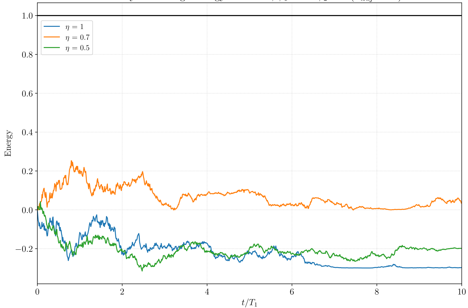
Homodyne: Average Energy over time, \phi_1 = 0 \phi_2 = 0 ( n_{\text{traj}} = 10 )
