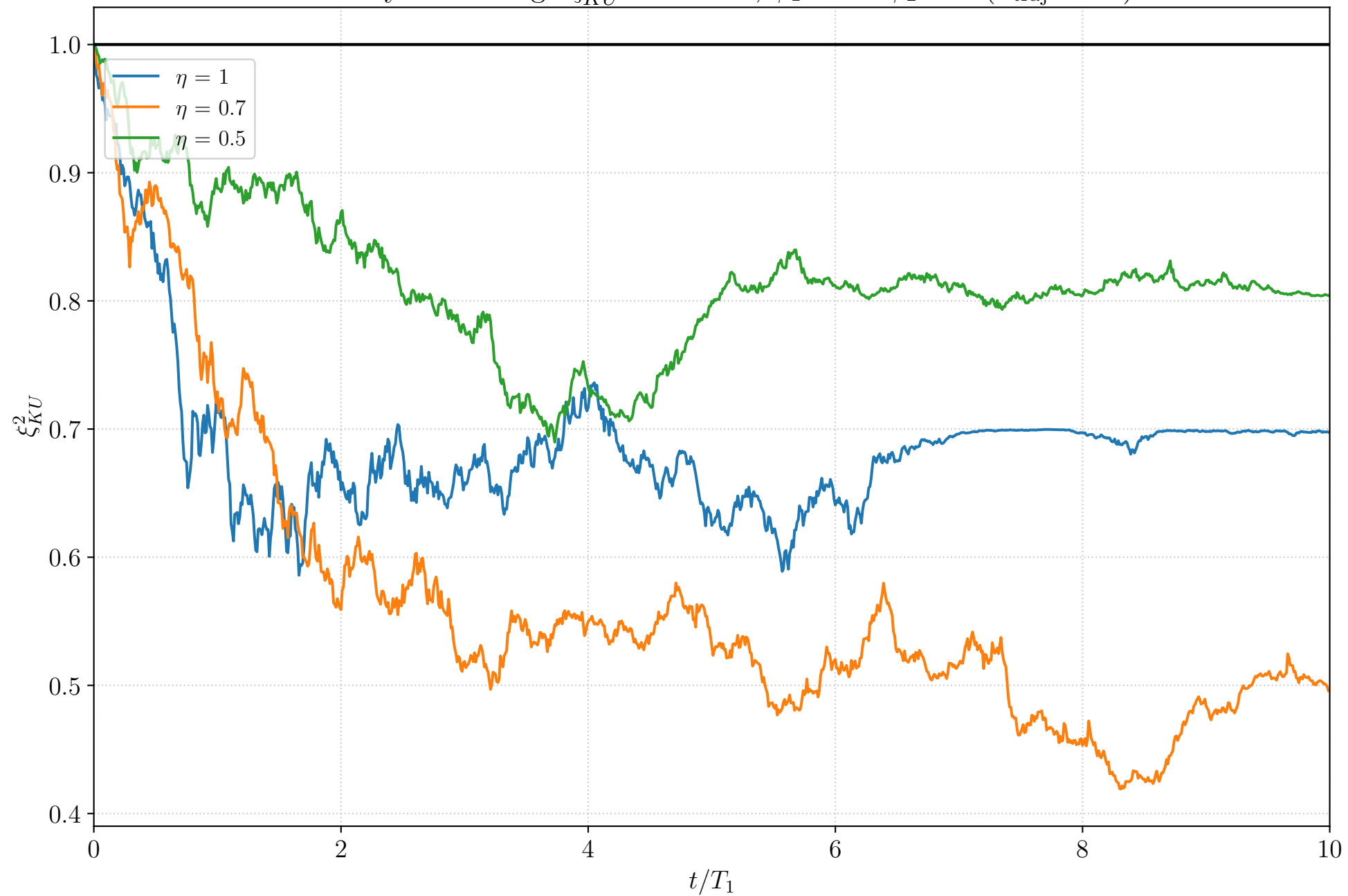
Homodyne: Average \xi_{KU}^2 over time, \phi_1 = 0 \phi_2 = 0 ( n_{\text{traj}} = 10 )
