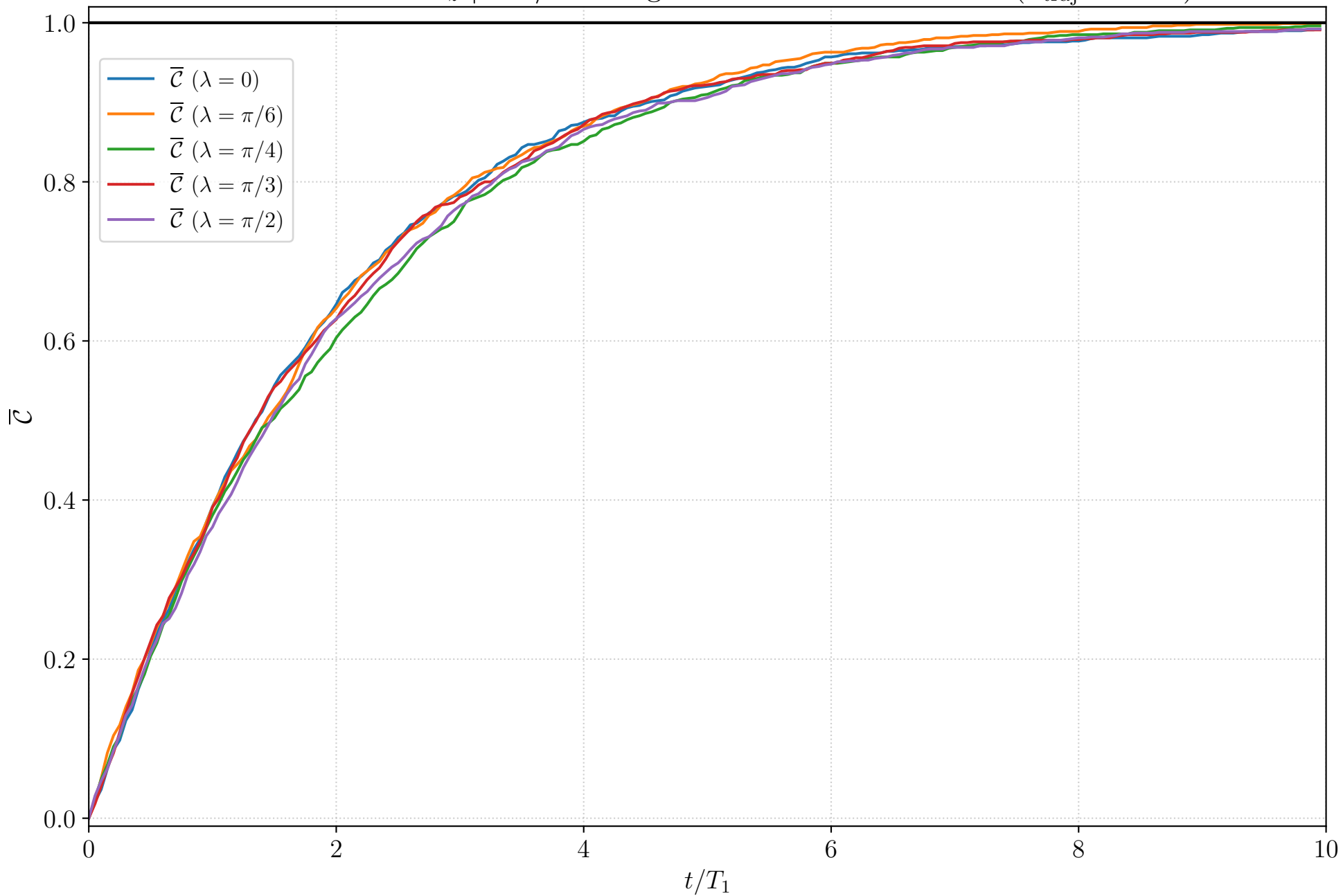
Photodetection J_z \mid ++ \rangle : Average concurrence \bar{\mathcal{C}} over time ( n_{\text{traj}} = 1000 )
