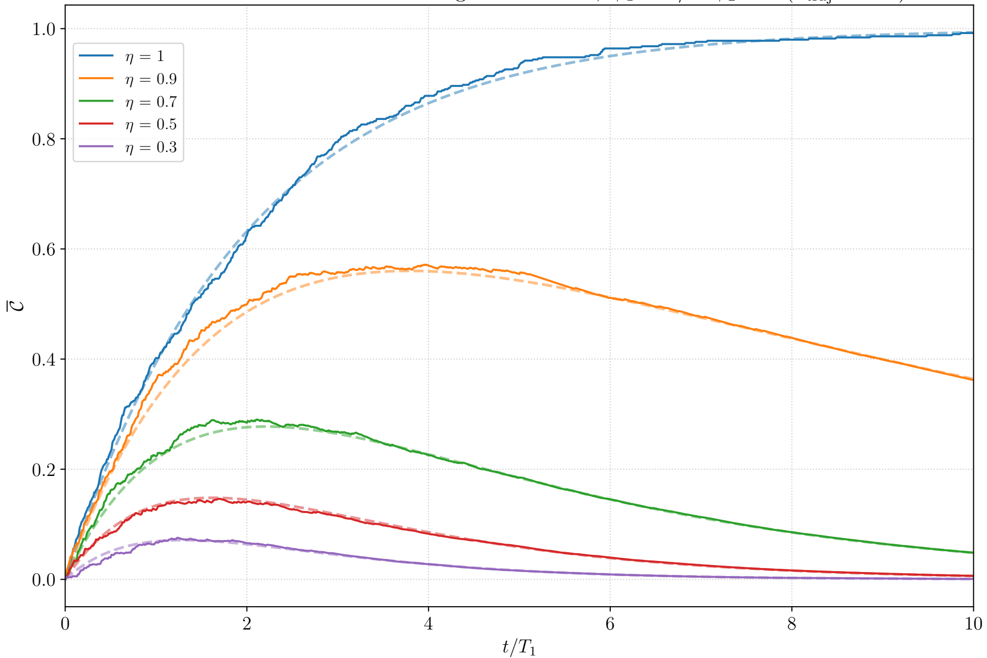
Inefficient Photodetection: Average \bar{\mathcal{C}} over time, \phi_1 = \pi/2 \phi_2 = 0 ( n_{\text{traj}} = 500 )
