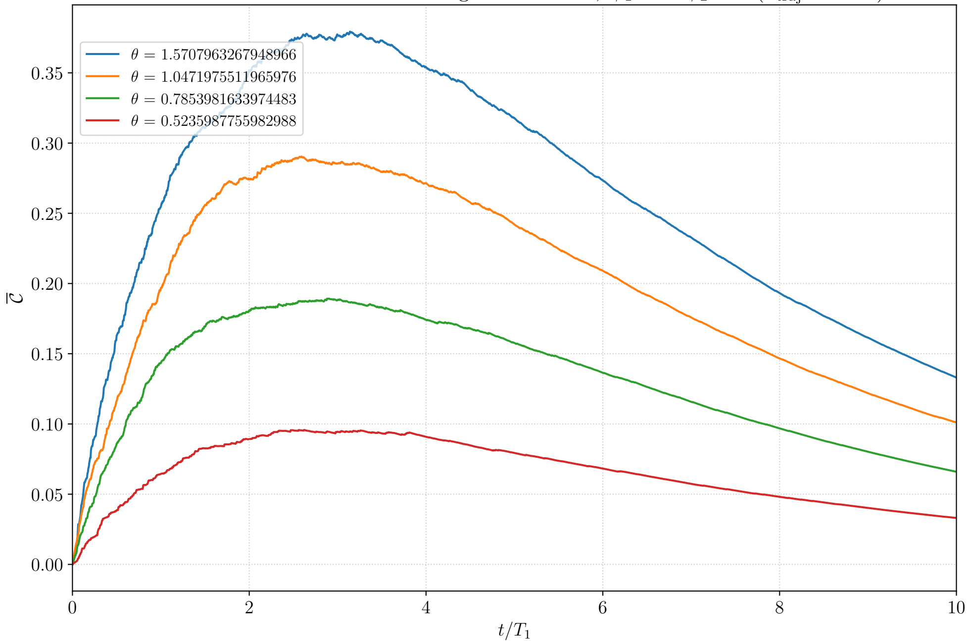
Inefficient Photodetection: Average \bar{\mathcal{C}} over time, \phi_1 = 0 \phi_2 = 0 ( n_{\text{traj}} = 1000 )
