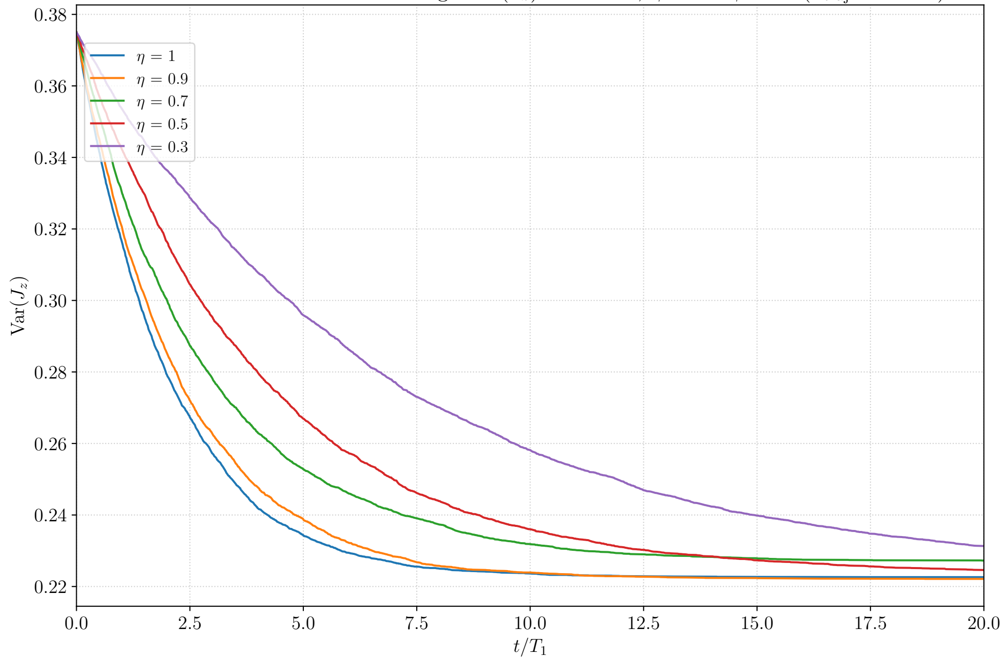
Inefficient Photodetection: Average \text{Var}(J_z) over time, \phi_1 = 0 \phi_2 = 0 ( n_{\text{traj}} = 10000 )
