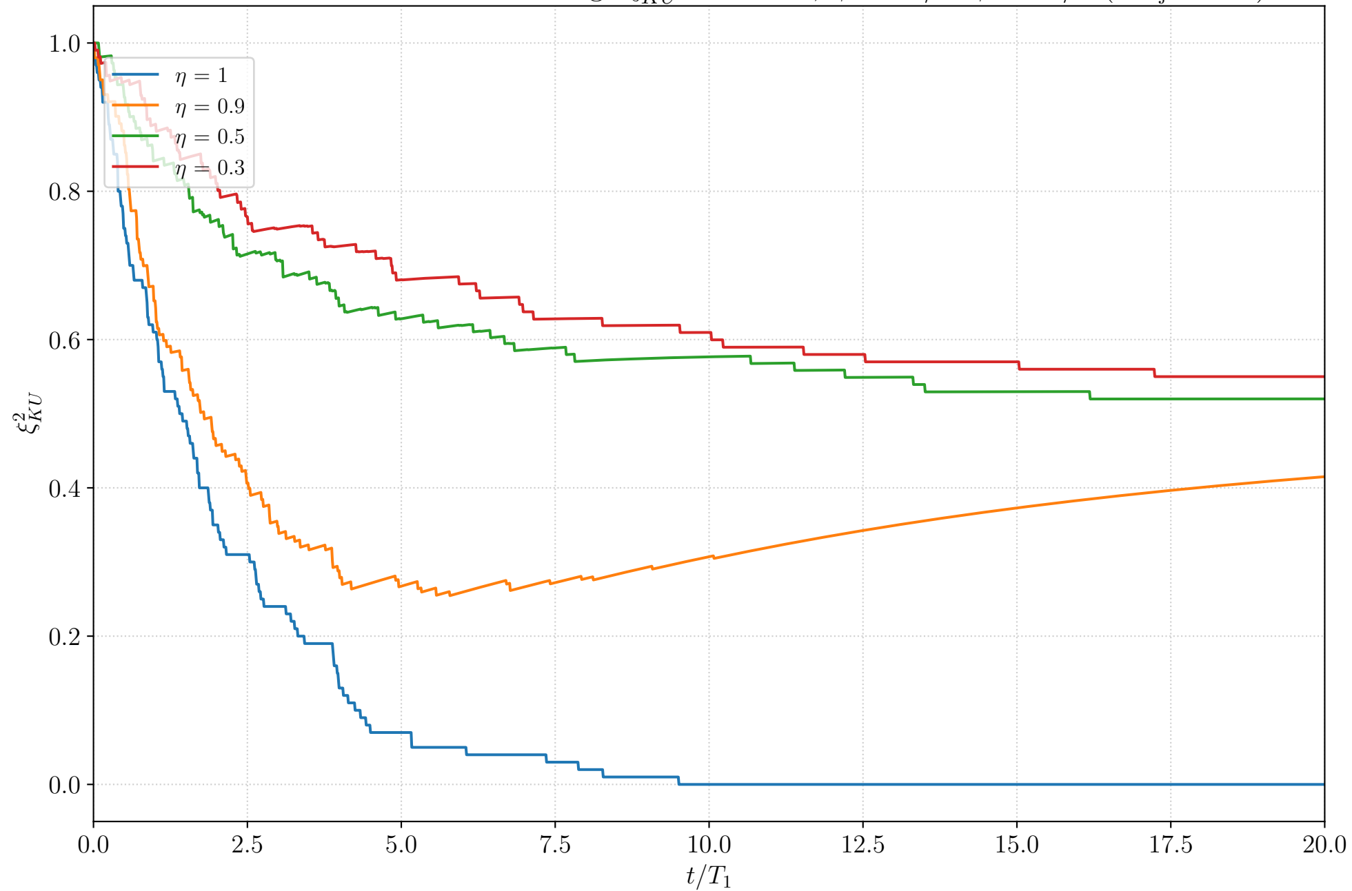
Inefficient Photodetection: Average \xi_{KU}^2 over time, \phi_1 = \pi/2 \phi_2 = \pi/2 ( n_{\text{traj}} = 100 )
