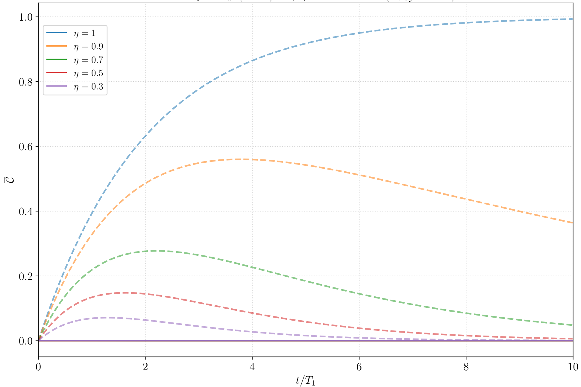
Homodyne J_z (N=2): \overline{\mathcal{C}} , \phi_1 = 0 \phi_2 = 0 ( n_{\text{traj}} = 100 )
