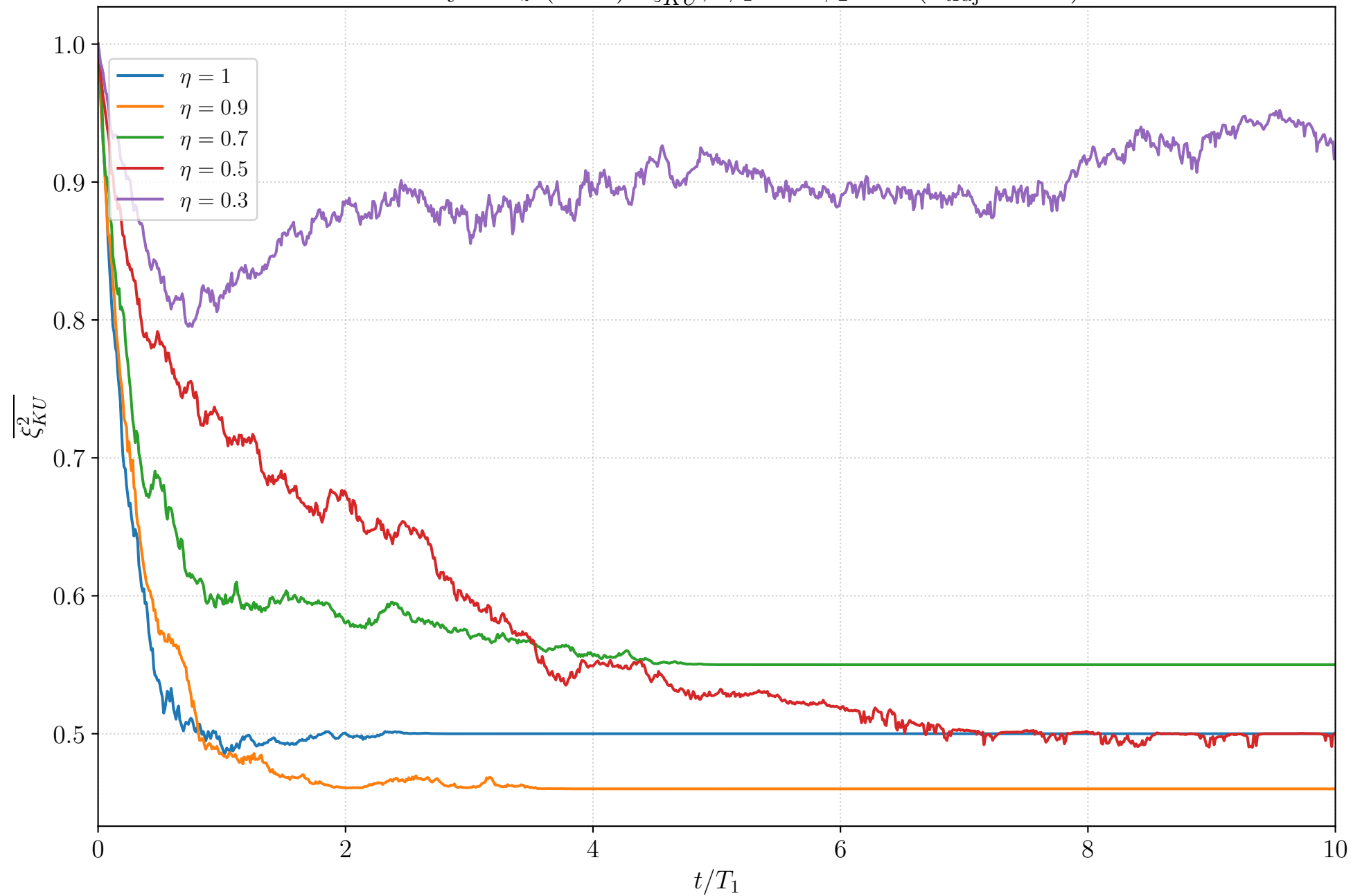
Homodyne J_z (N=2): \overline{\xi_{KU}^2} , \phi_1 = 0 \phi_2 = 0 ( n_{\text{traj}} = 100 )
