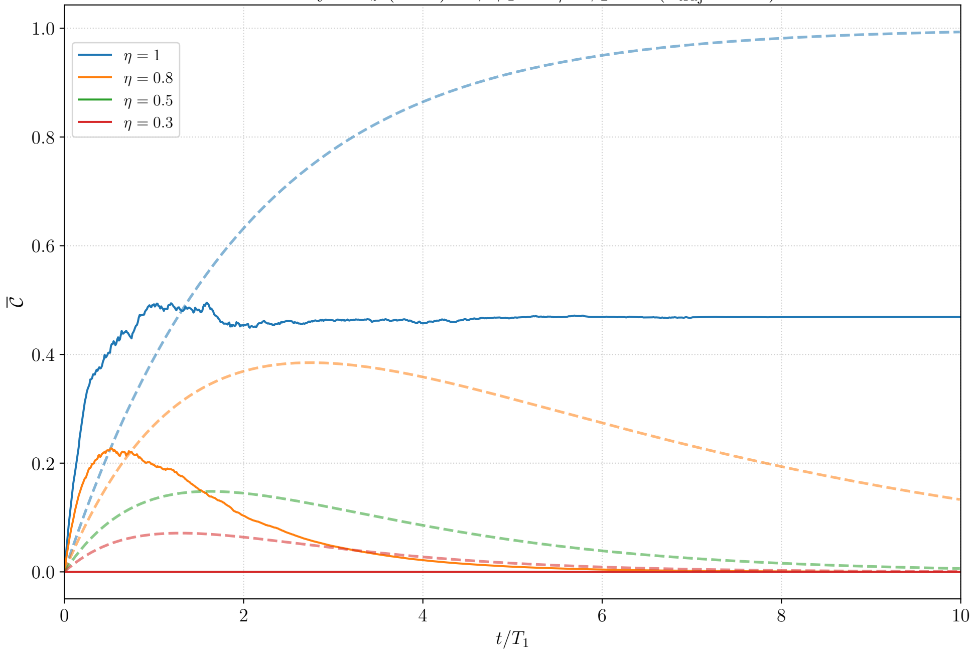
Homodyne J_z (N=2): \overline{\mathcal{C}} , \phi_1 = \pi/2 \phi_2 = 0 ( n_{\text{traj}} = 100 )
