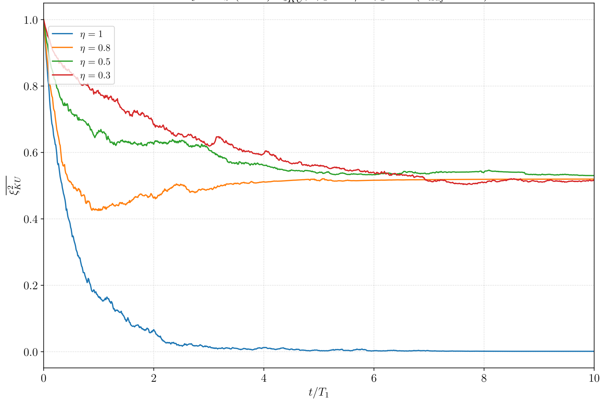
Homodyne J_z (N=2): \overline{\xi_{KU}^2} , \phi_1 = \pi/2 \phi_2 = 0 ( n_{\text{traj}} = 100 )
