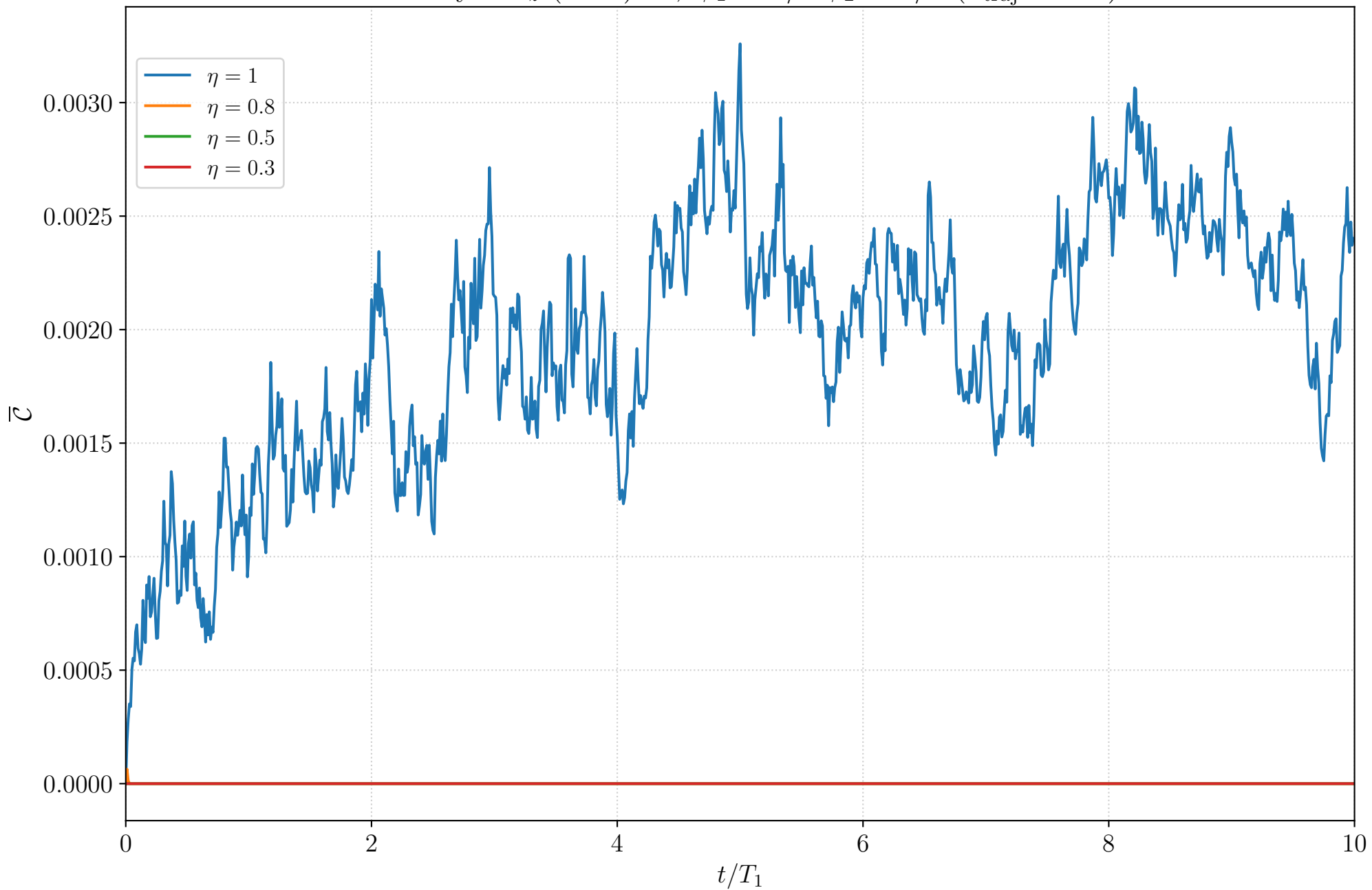
Homodyne J_z (N=2): \overline{\mathcal{C}} , \phi_1 = \pi/2 \phi_2 = \pi/2 ( n_{\text{traj}} = 100 )
