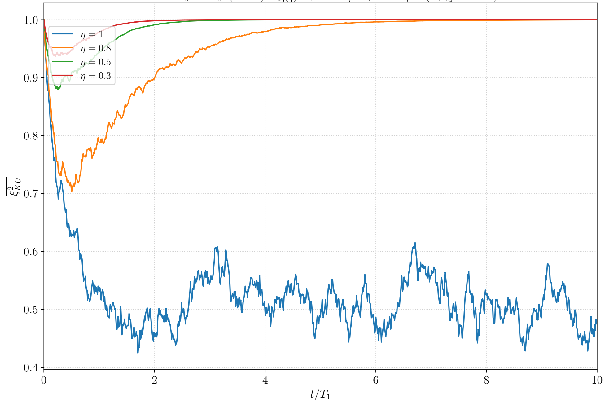
Homodyne J_z (N=2): \overline{\xi_{KU}^2} , \phi_1 = \pi/2 \phi_2 = \pi/2 ( n_{\text{traj}} = 100 )
