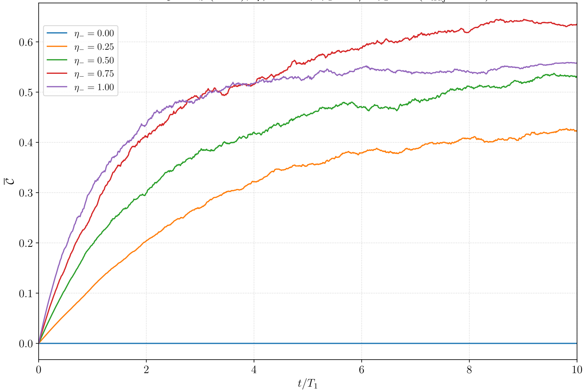
Homodyne J_z (N=2), \eta_+ = 1 : \bar{\mathcal{C}} , \phi_1 = \pi/2 \phi_2 = 0 ( n_{\text{traj}} = 100 )
