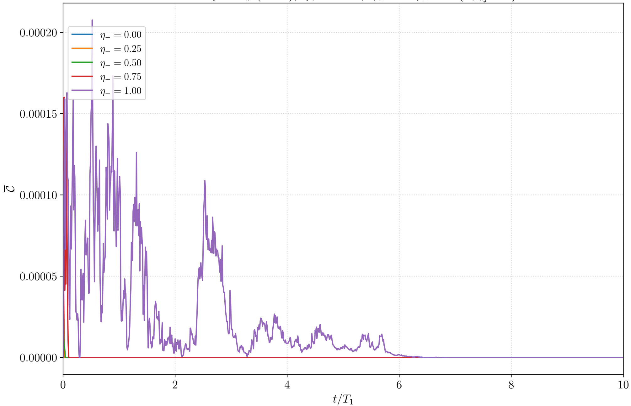
Homodyne J_z ( N=2 ), \eta_+ = 1 : \overline{\mathcal{C}} , \phi_1 = 0 \phi_2 = 0 ( n_{\text{traj}}=30 )
