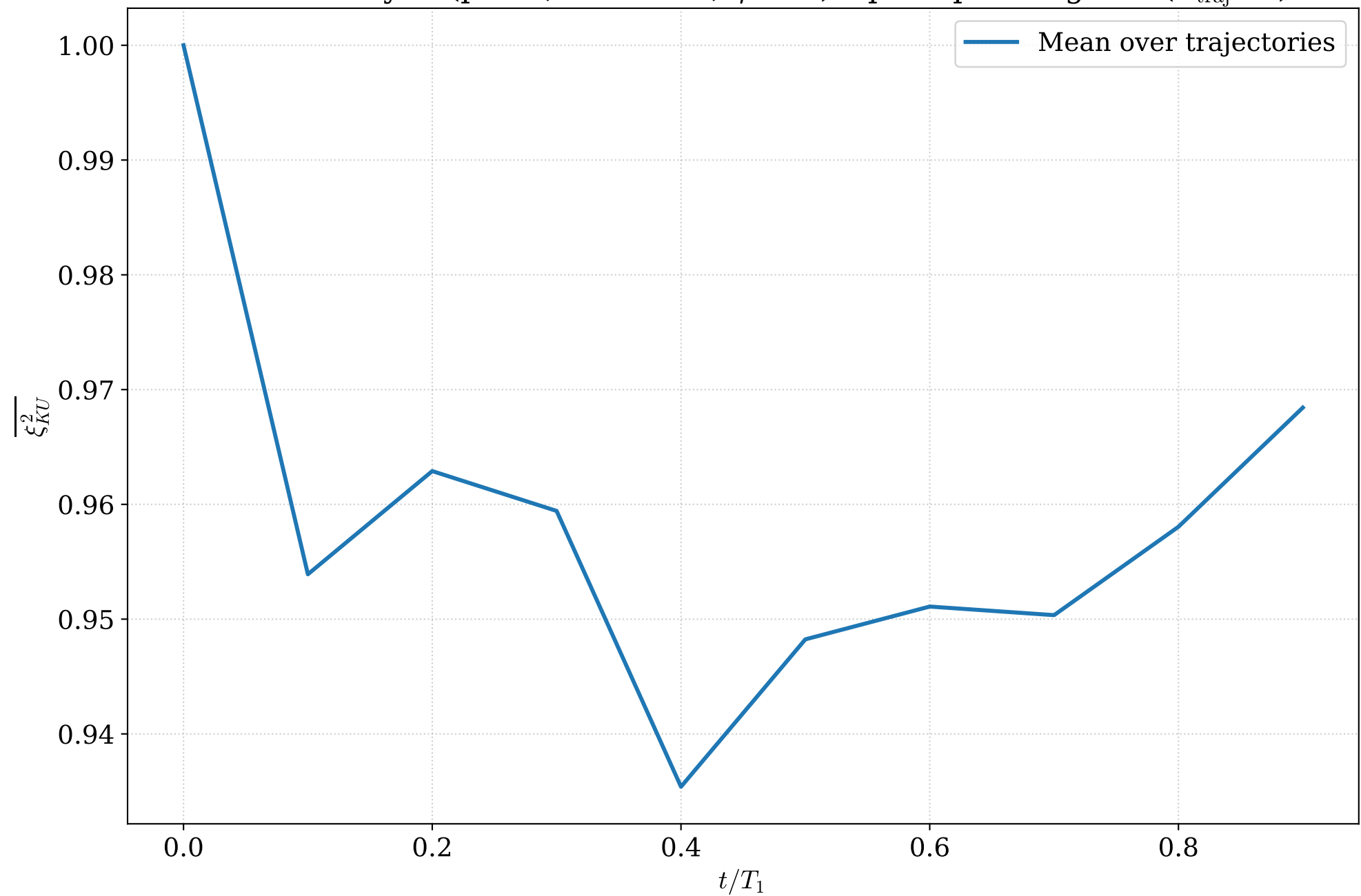
N=3 homodyne (plus3, U=tritter, \eta=0.8 ): spin squeezing KU ( n_{\text{traj}}=3 )
