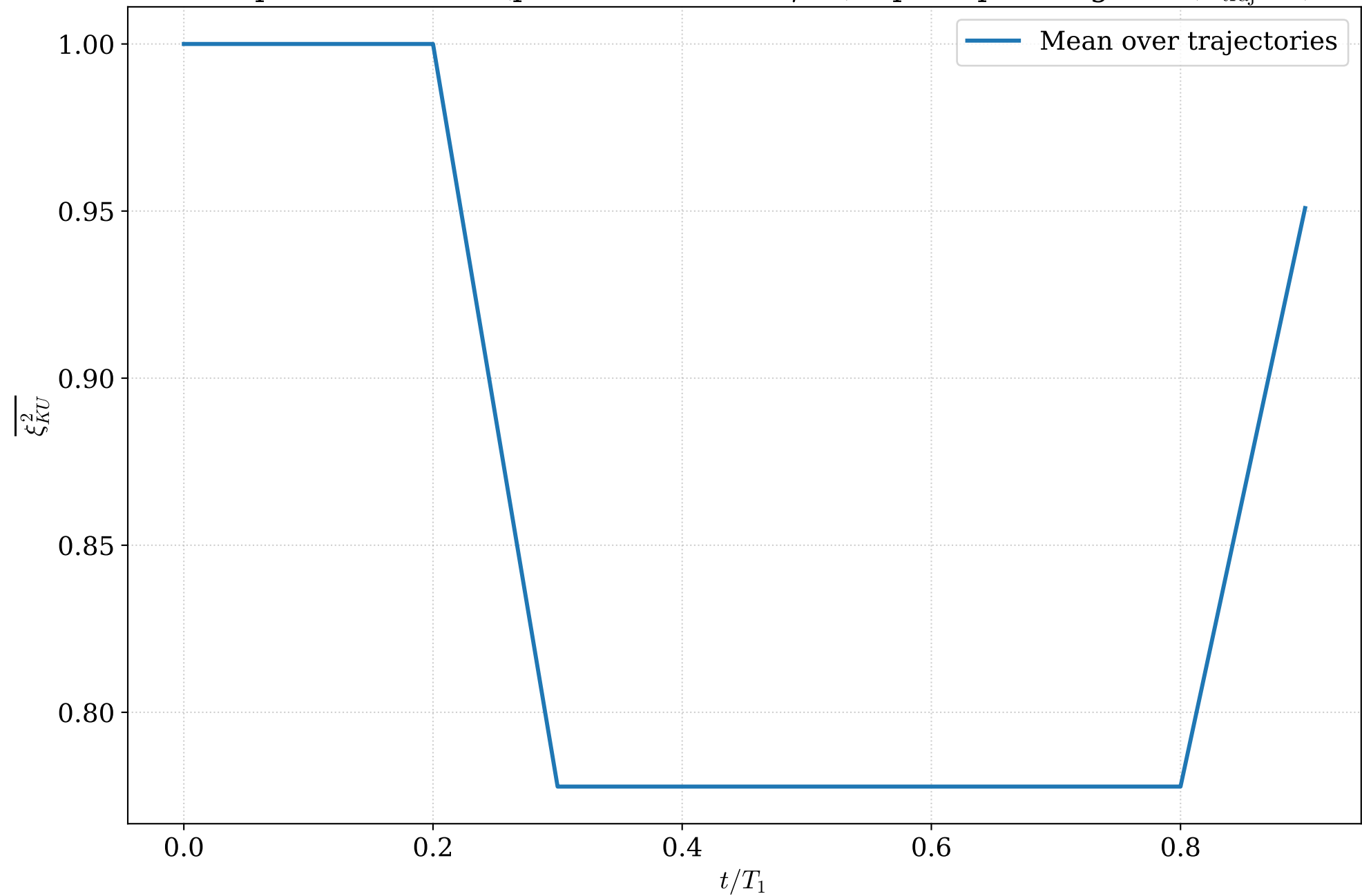
N=3 photodetection (plus3, U=tritter, \eta=1 ): spin squeezing KU ( n_{\text{traj}}=3 )
