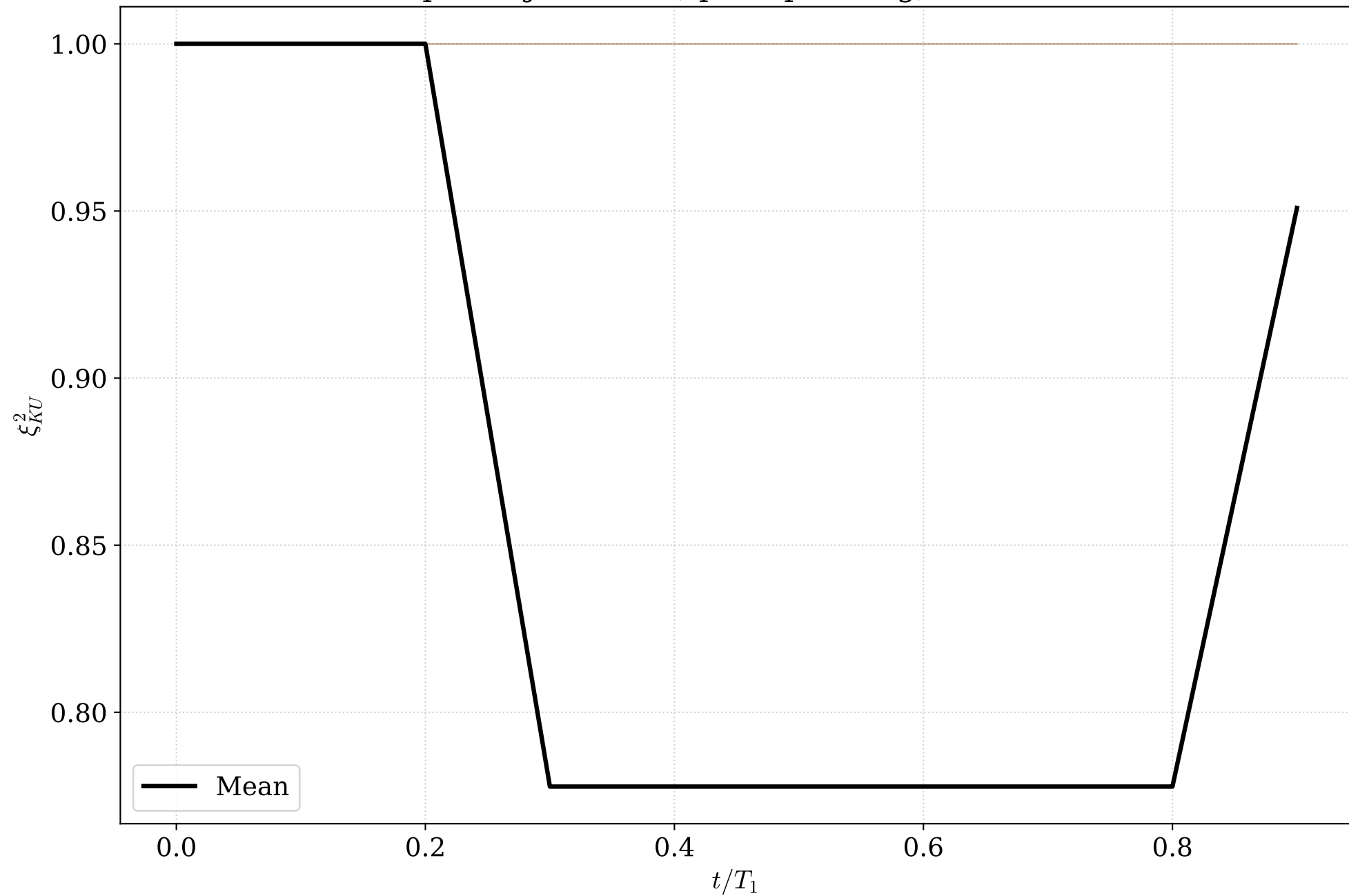
Sample trajectories (spin squeezing), first 2 runs
