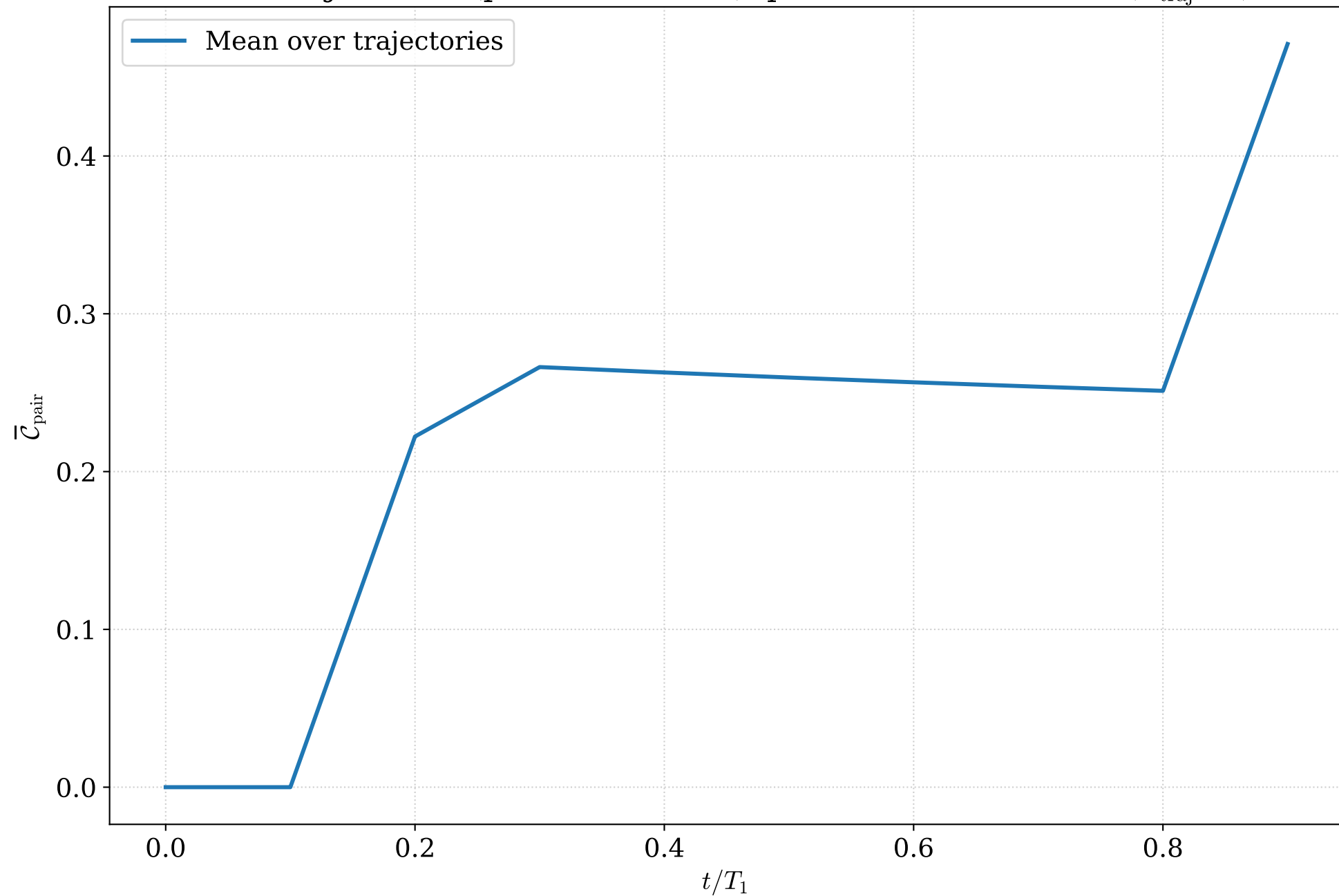
N=3 trajectories (plus3, U=tritter): pairwise concurrence ( n_{\text{traj}}=3 )
