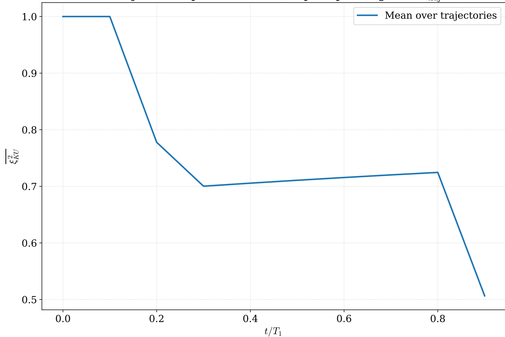
N=3 trajectories (plus3, U=tritter): spin squeezing KU ( n_{\text{traj}}=3 )
