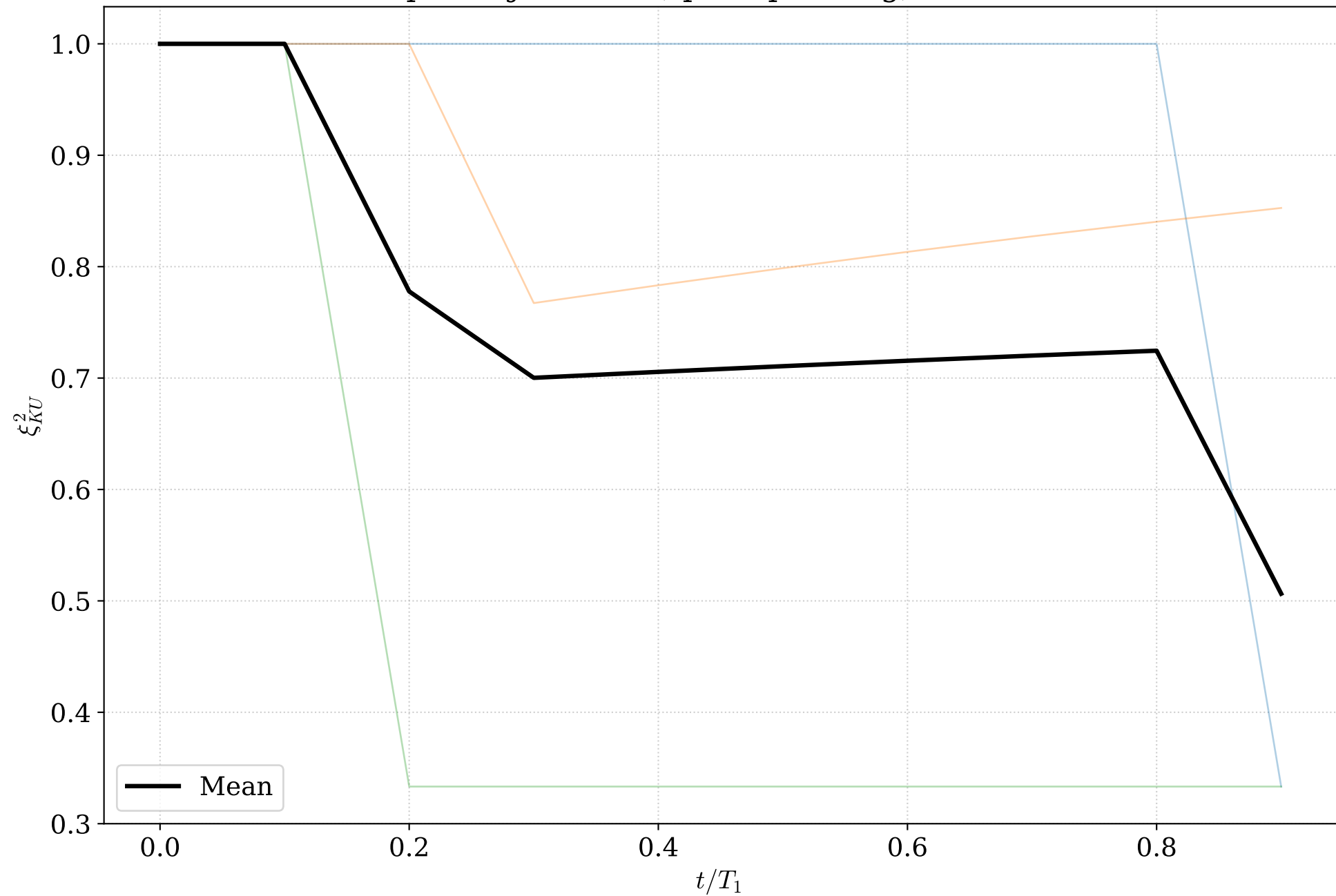
Sample trajectories (spin squeezing), first 3 runs
