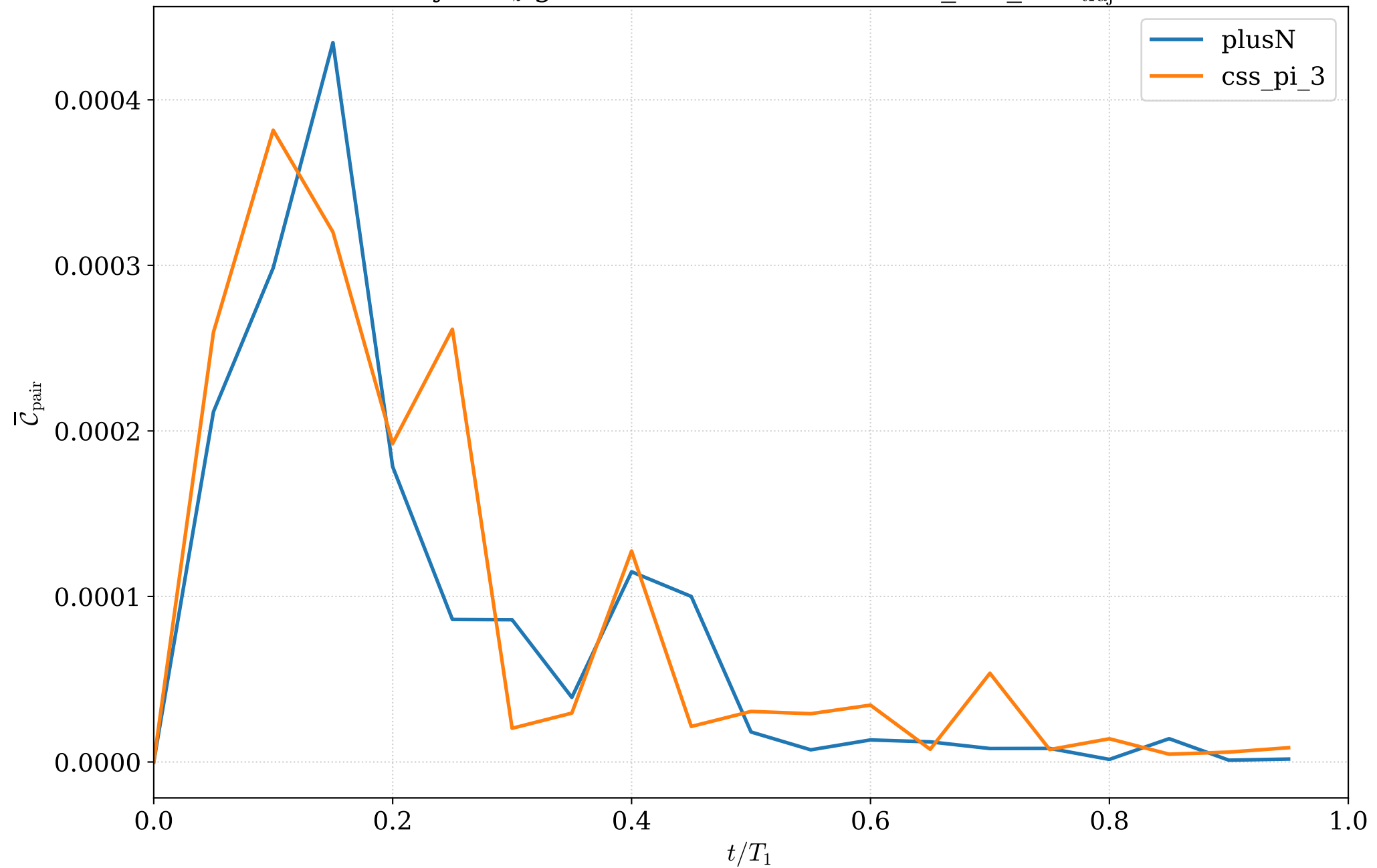
Homodyne J_z generic N=3 , U=\text{collective\_diff\_3} , n_{\text{traj}}=10
