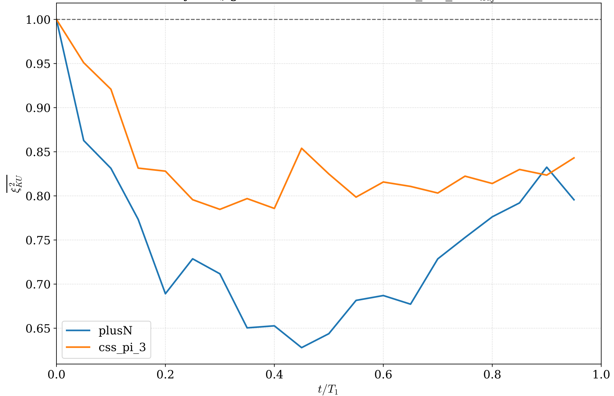
Homodyne J_z generic N=3, U=collective_diff_3, n traj =10
