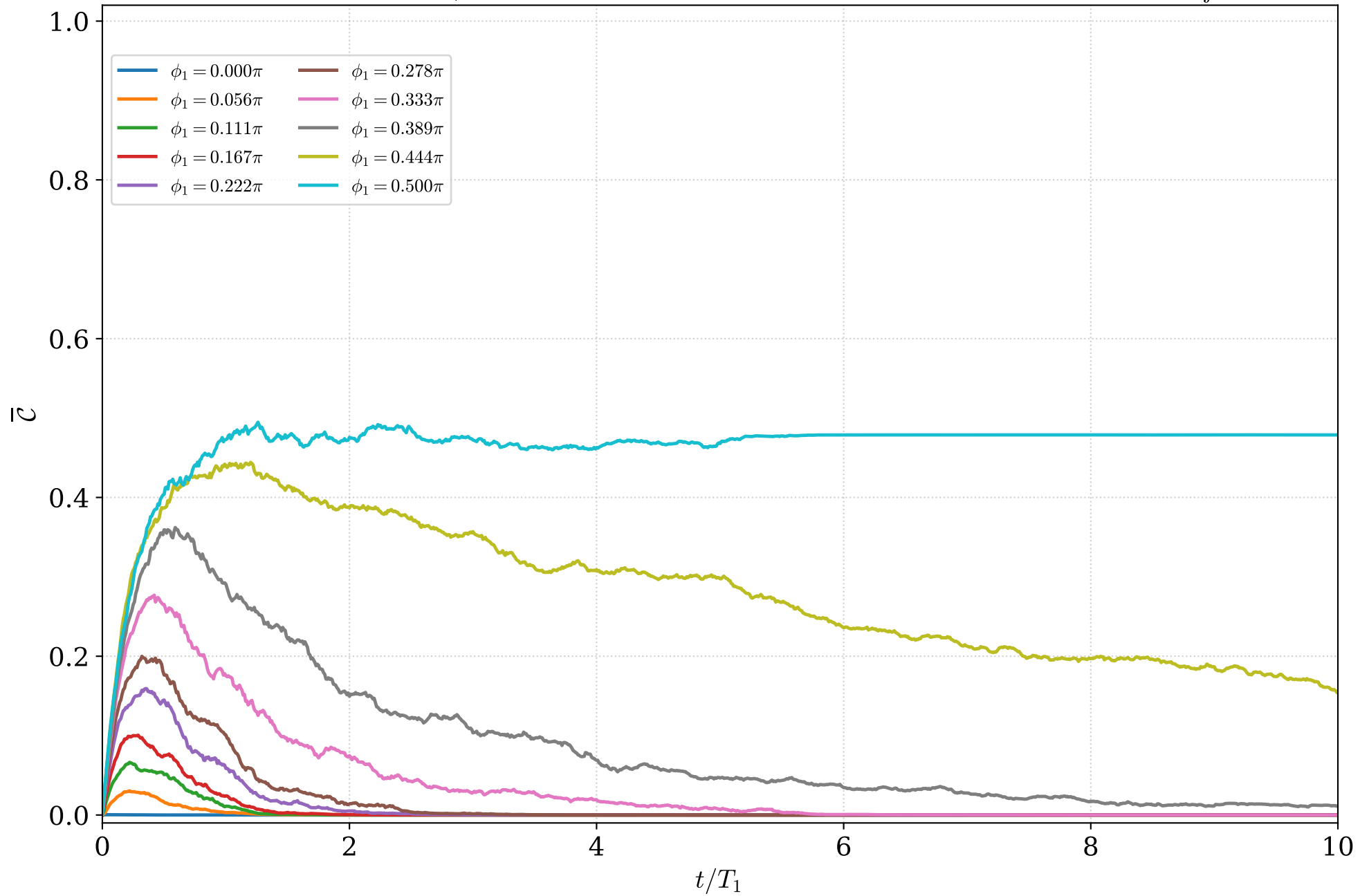
Homodyne J_z ( N=2, |++\rangle ): scan of \phi_1 , \phi_2=0 , \eta_+=1.00 , \eta_-=1.00 ( n_{\text{traj}}=100 )
