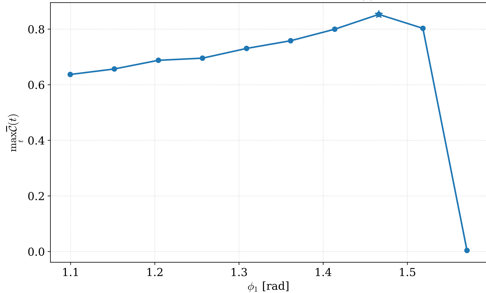
Best concurrence vs scanned \phi_1
