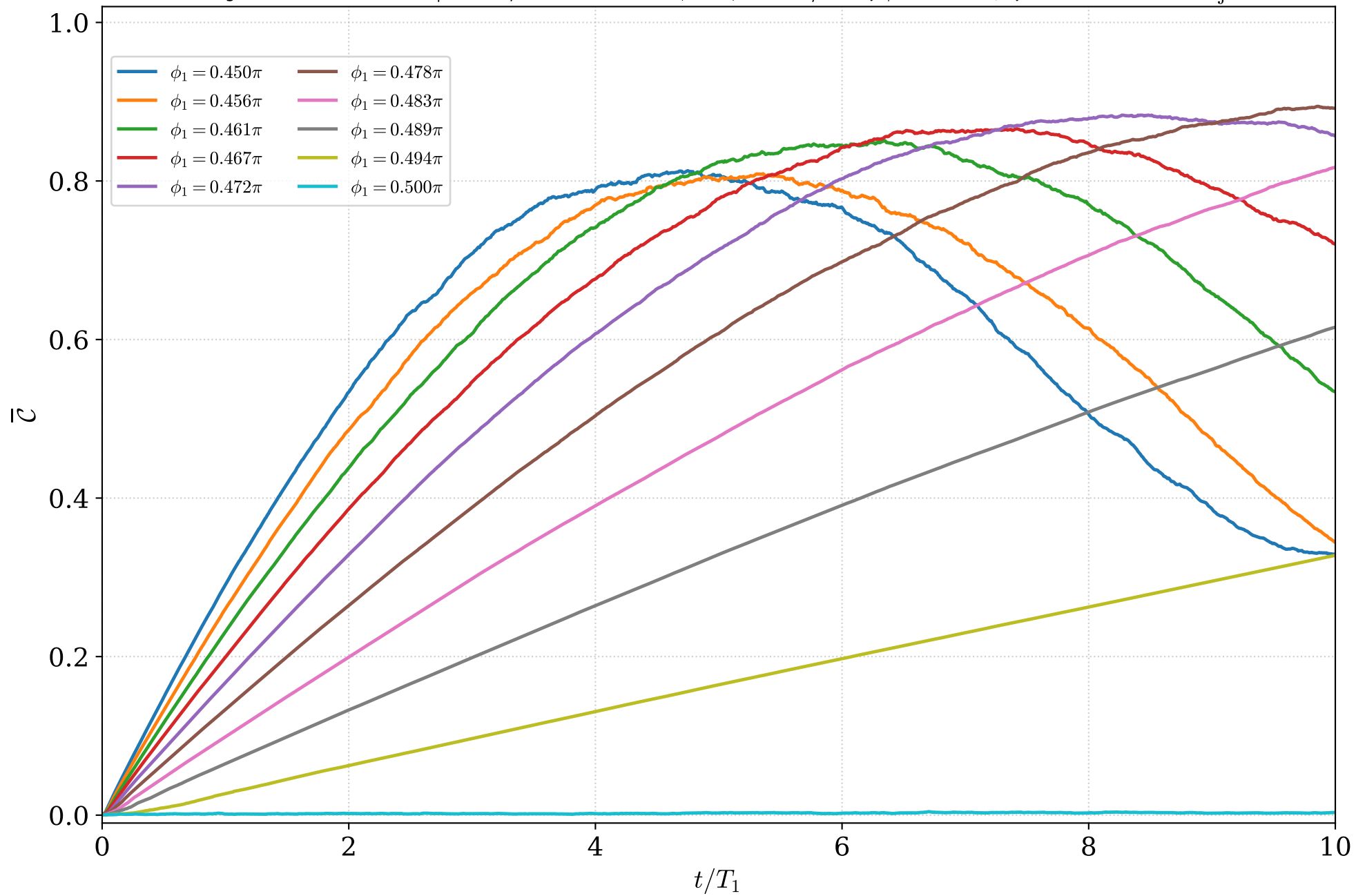
Homodyne J_z (N=2, |++\rangle ): scan of \phi_1 , \phi_2 = \pi/2 , \eta_+ = 1.00 , \eta_- = 1.00 ( n_{\text{traj}}=100 )
