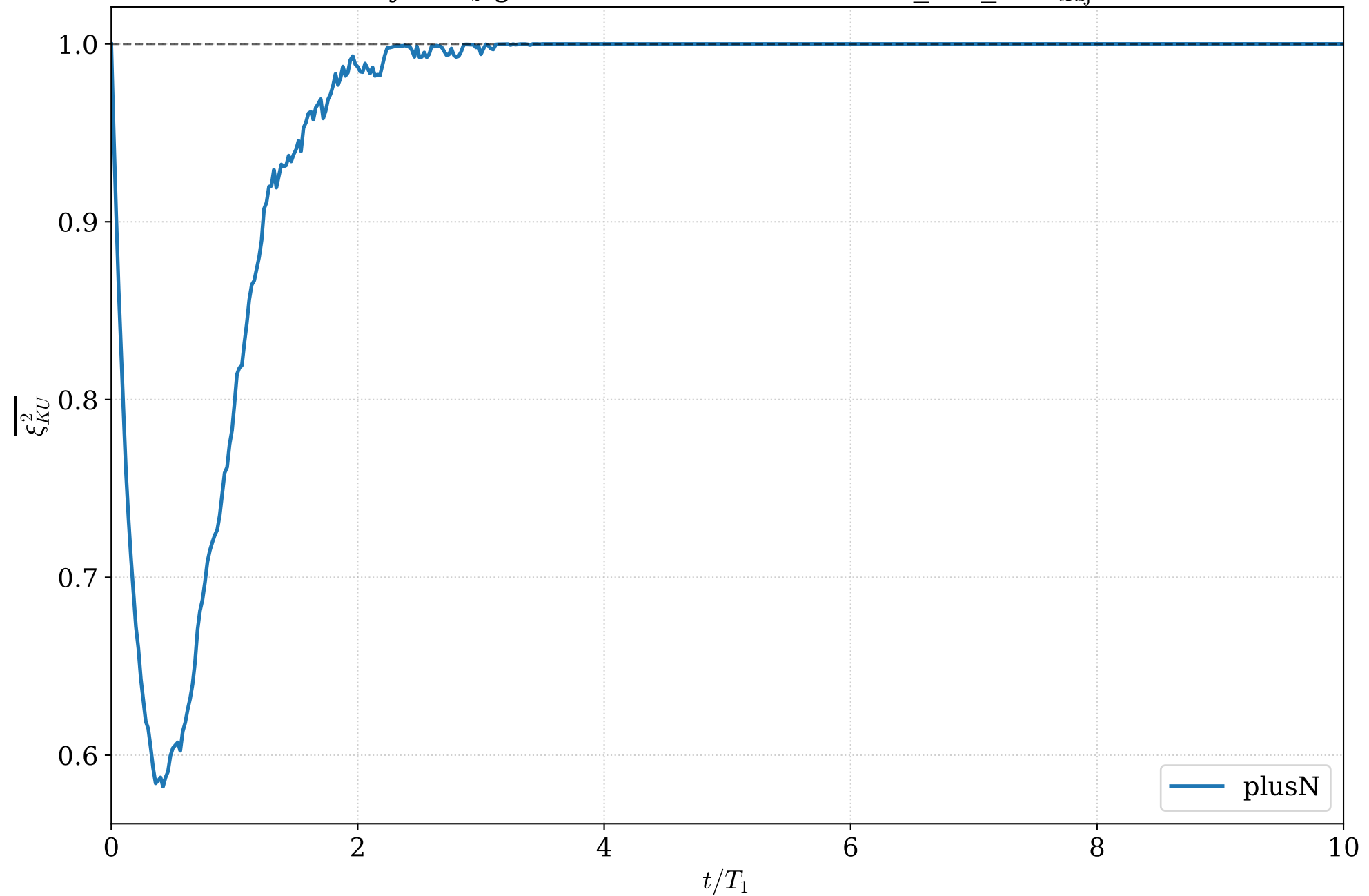
Homodyne J_z generic N=3, U=collective_diff_3, n traj =100
