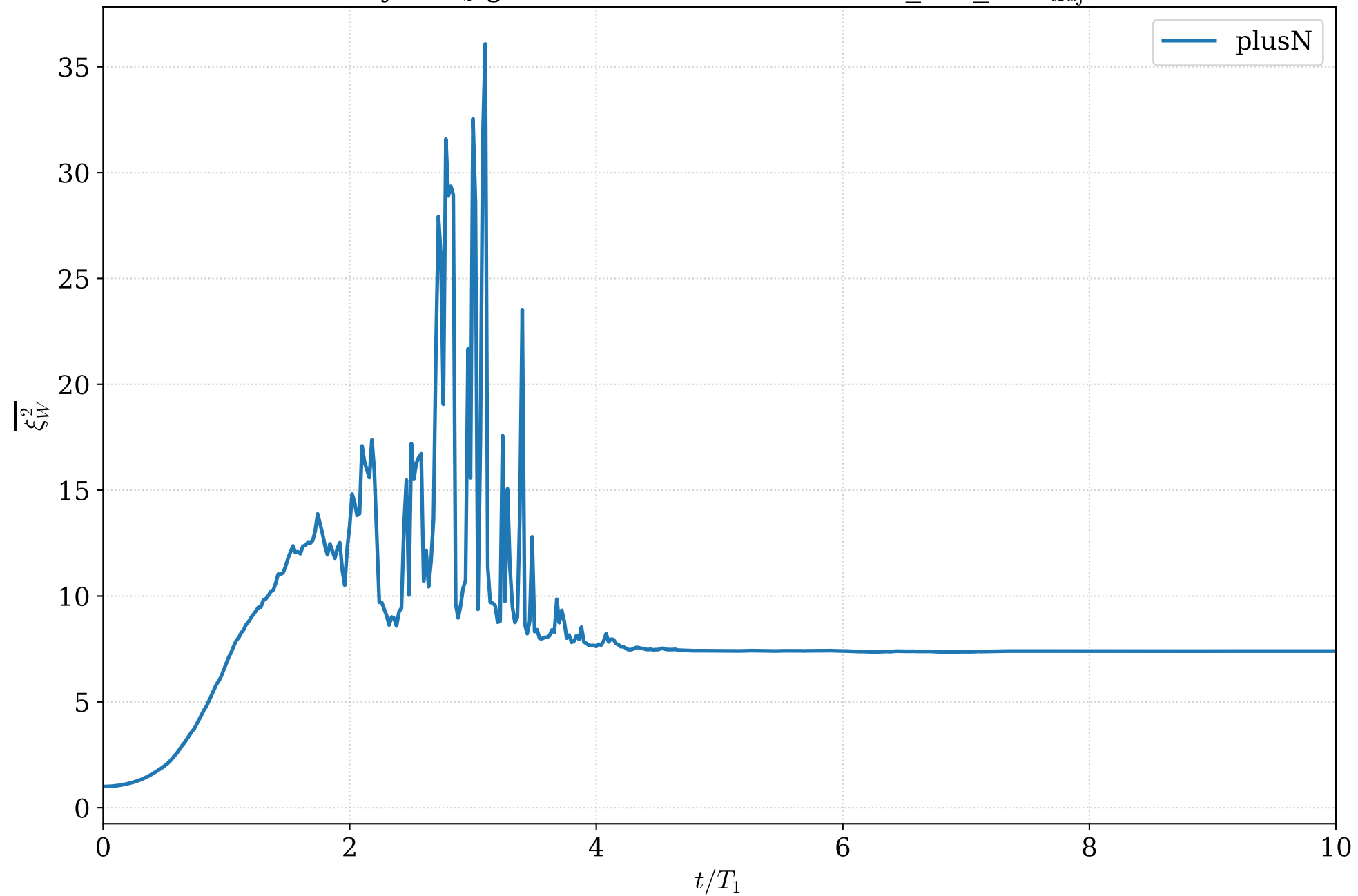
Homodyne J_z generic N=3 , U=\text{collective\_diff\_3} , n_{\text{traj}}=100
