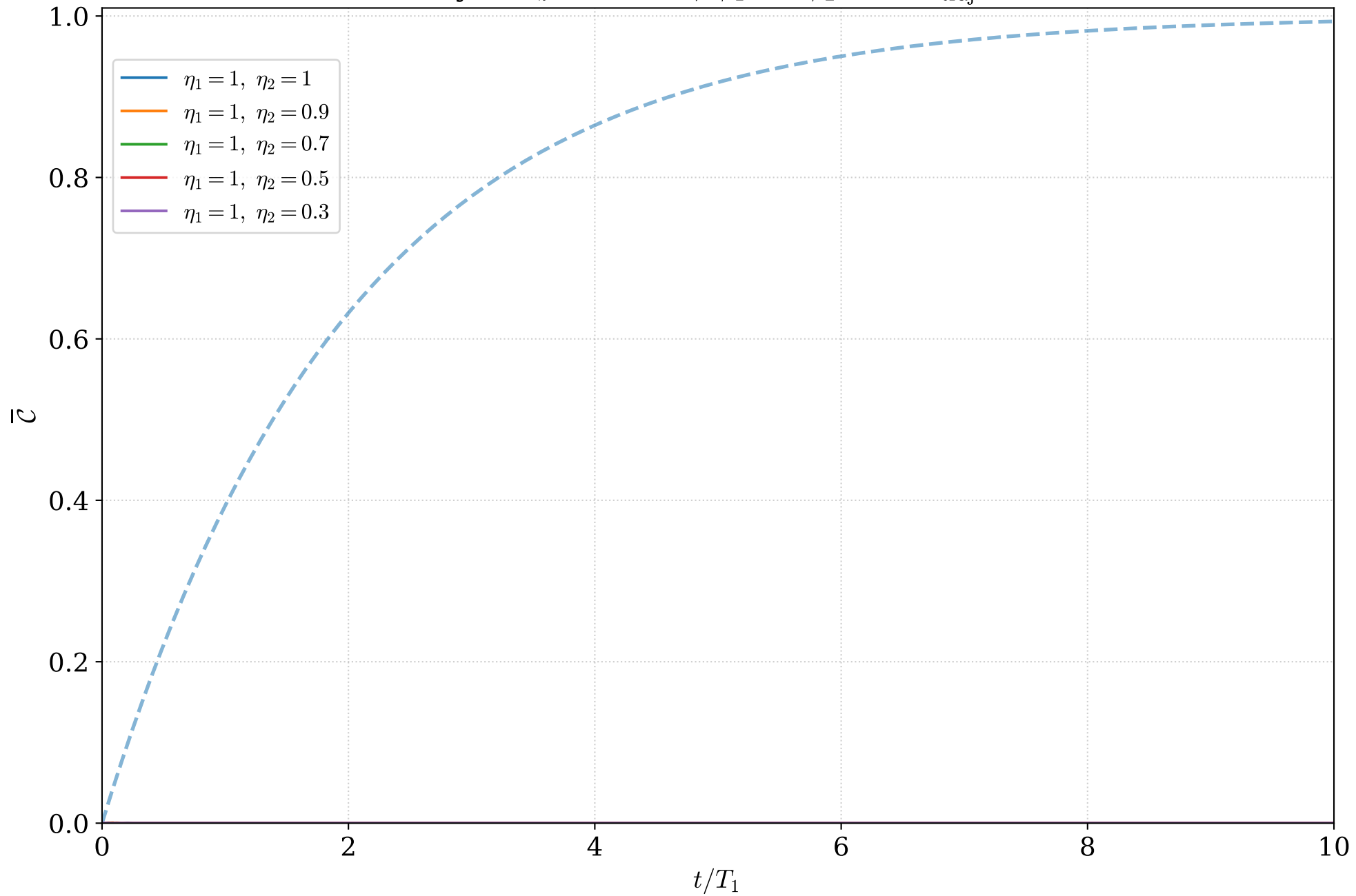
Homodyne J_z (N=2): \bar{\mathcal{C}} , \phi_1 = 0 \phi_2 = 0 ( n_{\text{traj}} = 100 )
