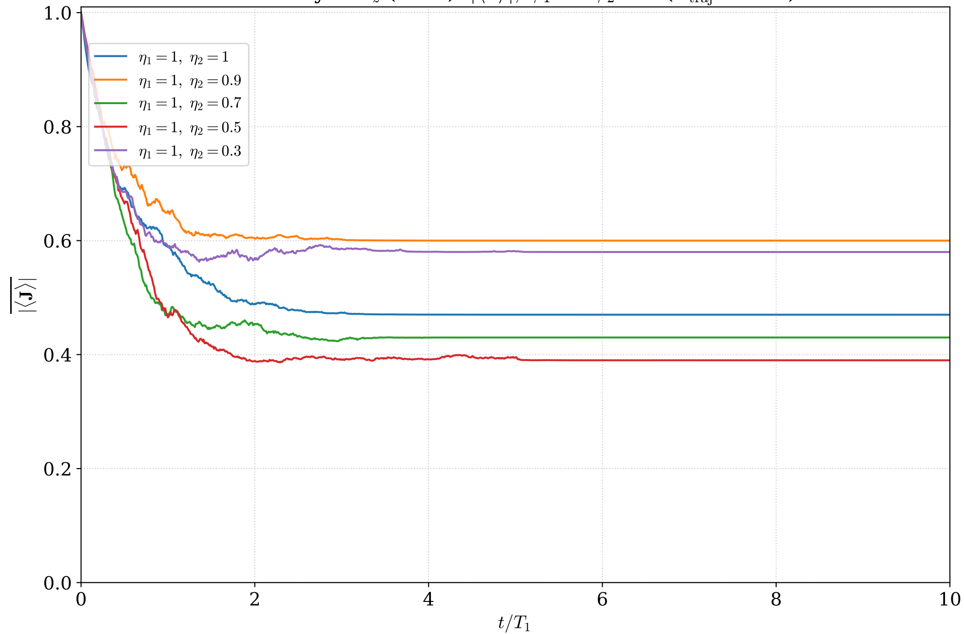
Homodyne J_z (N=2): |\overline{\langle \mathbf{J} \rangle}| , \phi_1 = 0 \phi_2 = 0 ( n_{\text{traj}} = 100 )
