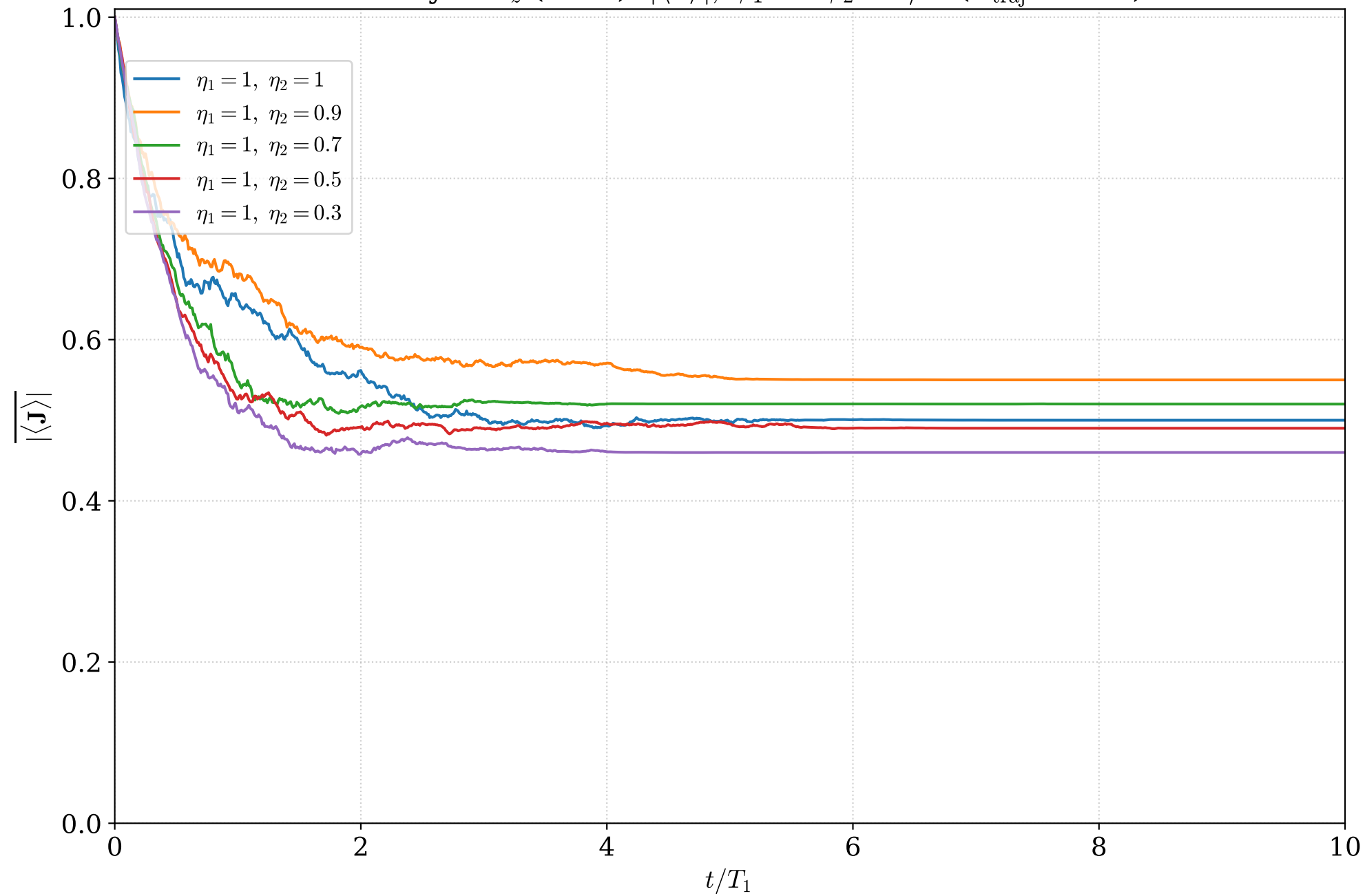
Homodyne J_z (N=2): |\overline{\langle \mathbf{J} \rangle}| , \phi_1 = 0 \phi_2 = \pi/2 ( n_{\text{traj}} = 100 )
