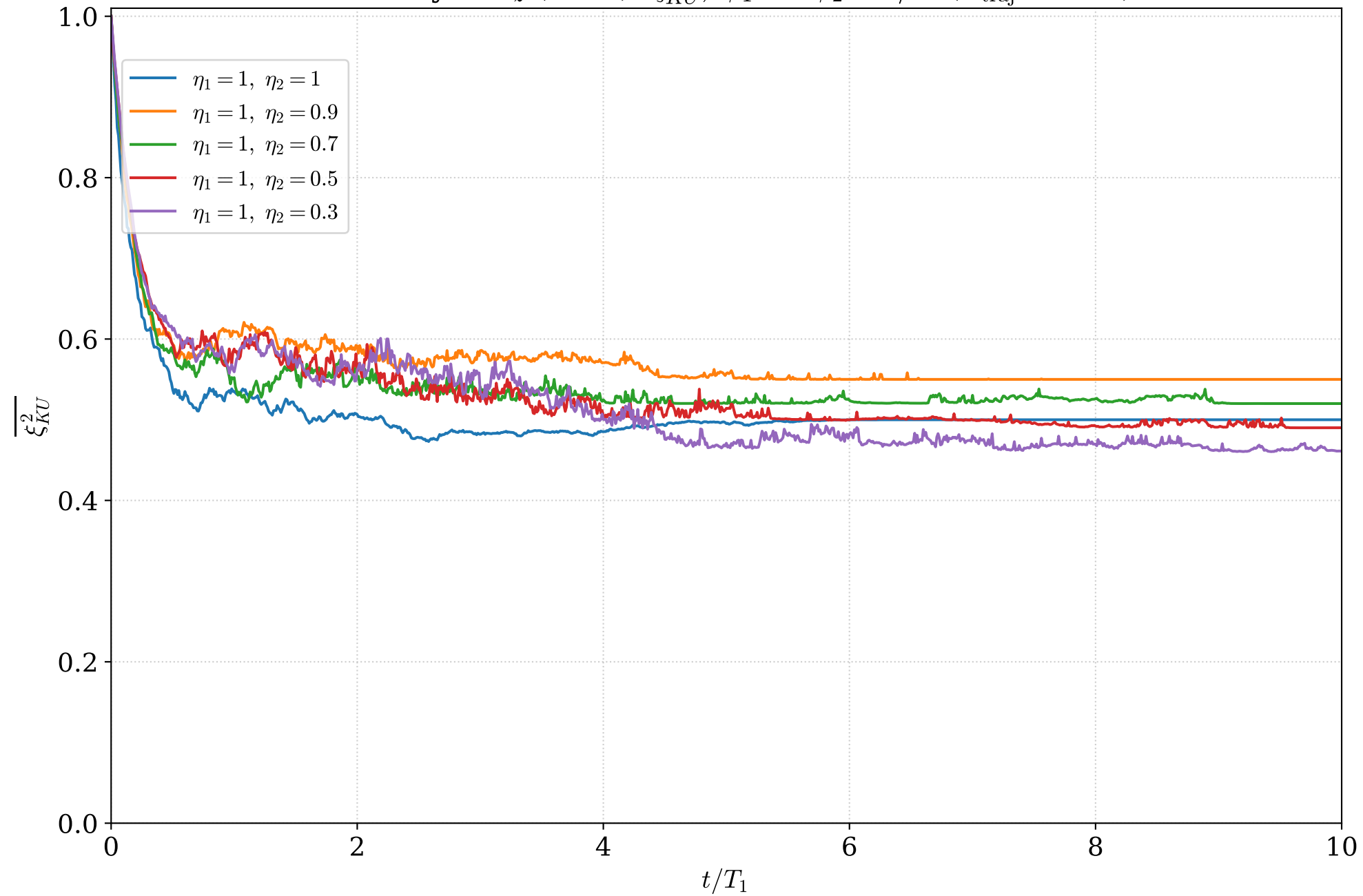
Homodyne J_z (N=2): \overline{\xi_{KU}^2} , \phi_1 = 0 \phi_2 = \pi/2 ( n_{\text{traj}} = 100 )
