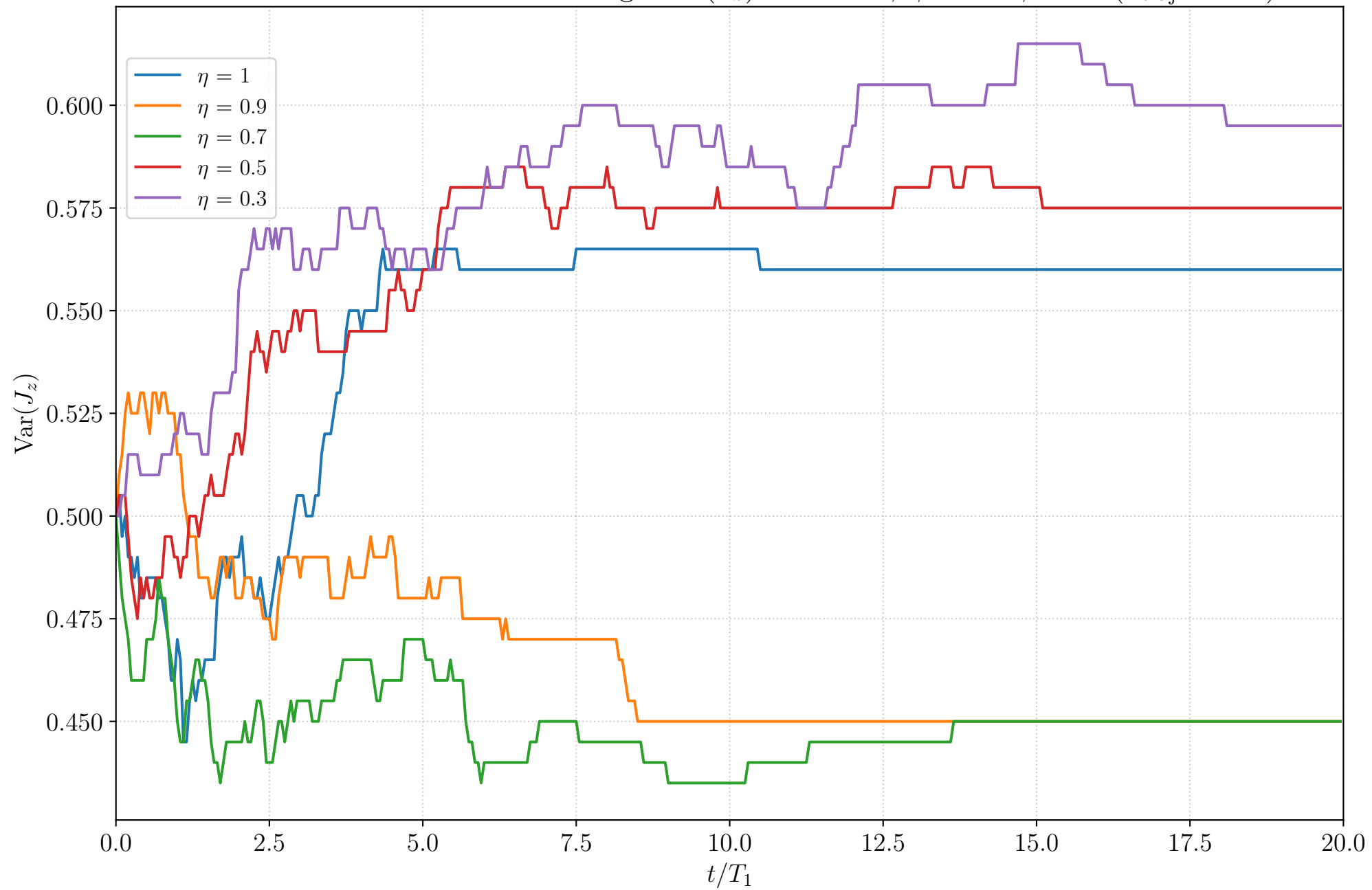
Inefficient Photodetection: Average \text{Var}(J_z) over time, \phi_1 = 0 \phi_2 = 0 ( n_{\text{traj}} = 100 )
