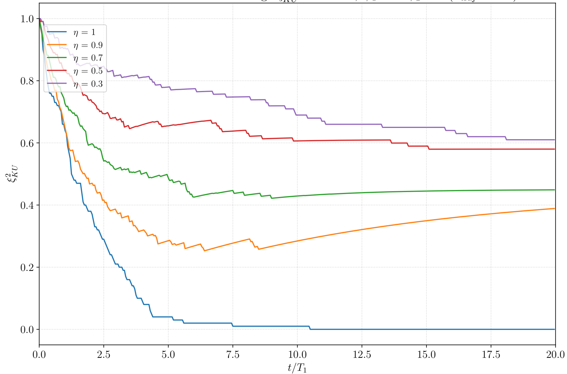
Inefficient Photodetection: Average \xi_{KU}^2 over time, \phi_1 = 0 \phi_2 = 0 ( n_{\text{traj}} = 100 )
