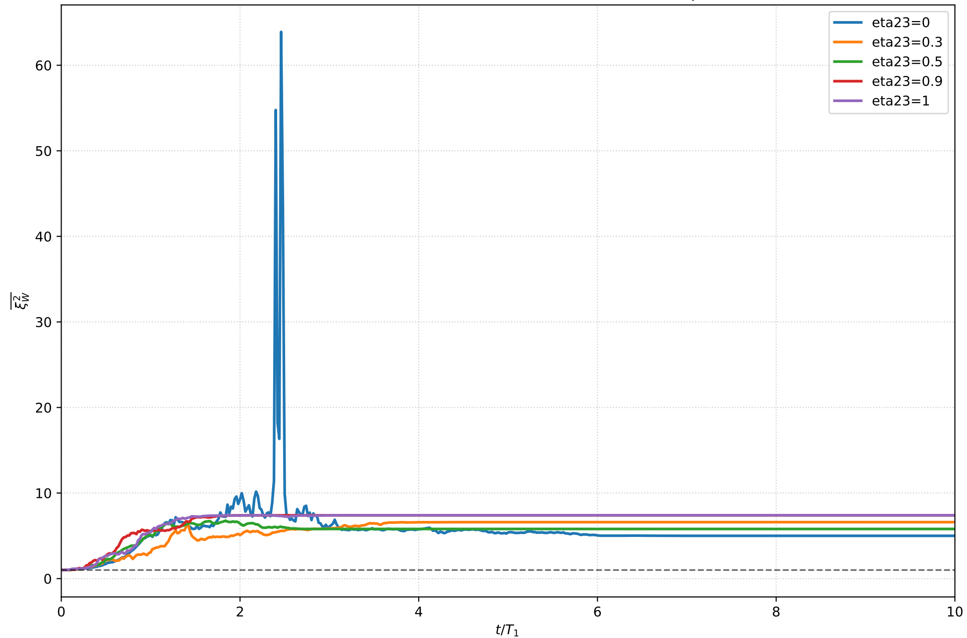
Homodyne N=3, state=plusplus, U=collective_diff_3, n traj =10, \eta_1=1
