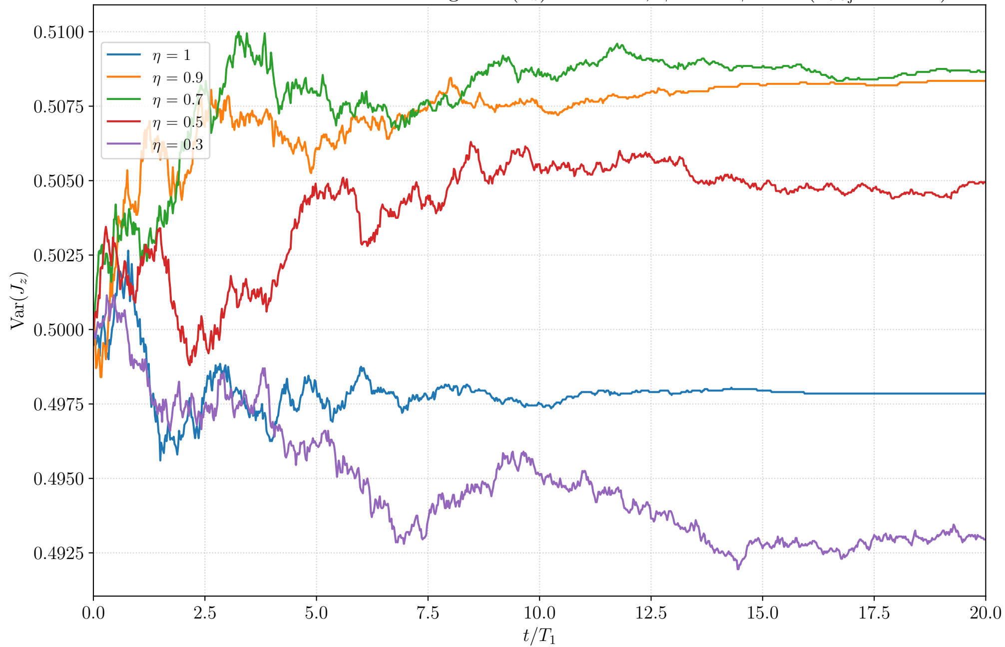
Inefficient Photodetection: Average \text{Var}(J_z) over time, \phi_1 = 0 \phi_2 = 0 ( n_{\text{traj}} = 10000 )
