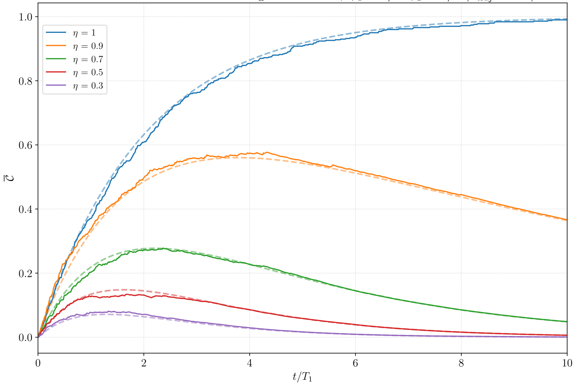
Inefficient Photodetection: Average \bar{\mathcal{C}} over time, \phi_1 = \pi/2 \phi_2 = \pi/2 ( n_{\text{traj}} = 500 )
