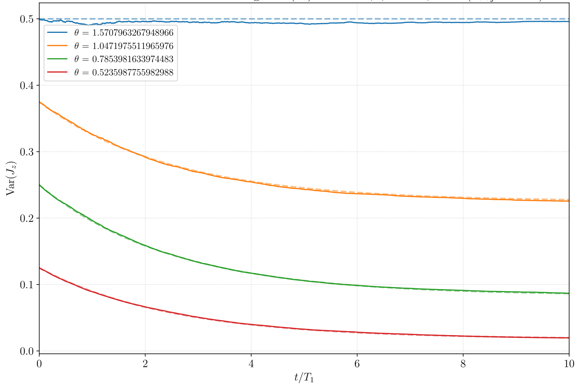
Inefficient Photodetection: Average \text{Var}(J_z) over time, \phi_1 = 0 \phi_2 = 0 ( n_{\text{traj}} = 5000 )
