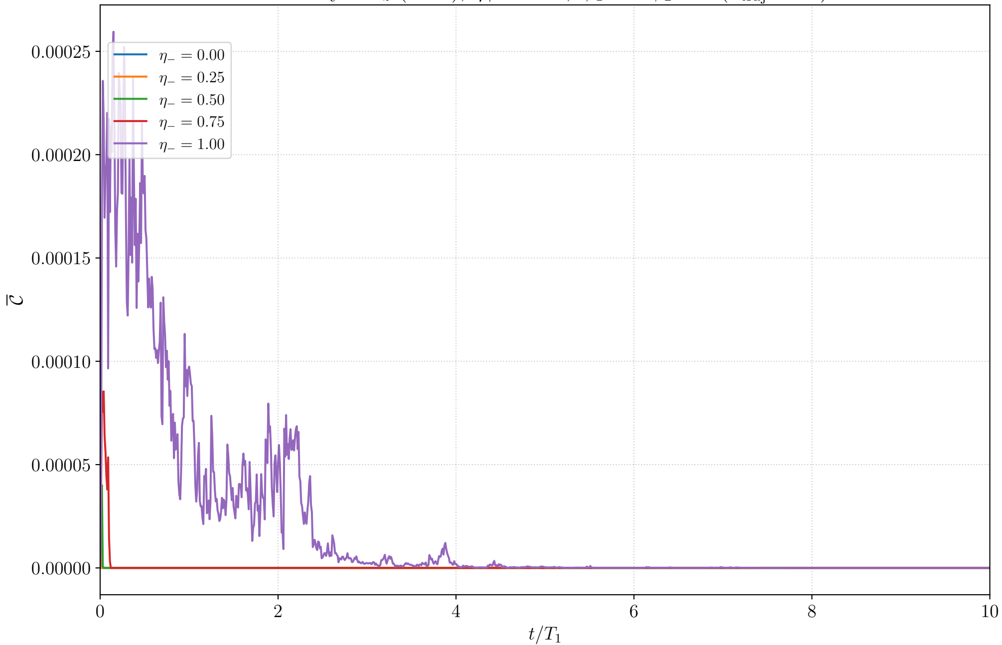
Homodyne J_z (N=2), \eta_+ = 1 : \overline{\mathcal{C}} , \phi_1 = 0 \phi_2 = 0 ( n_{\text{traj}} = 50 )
