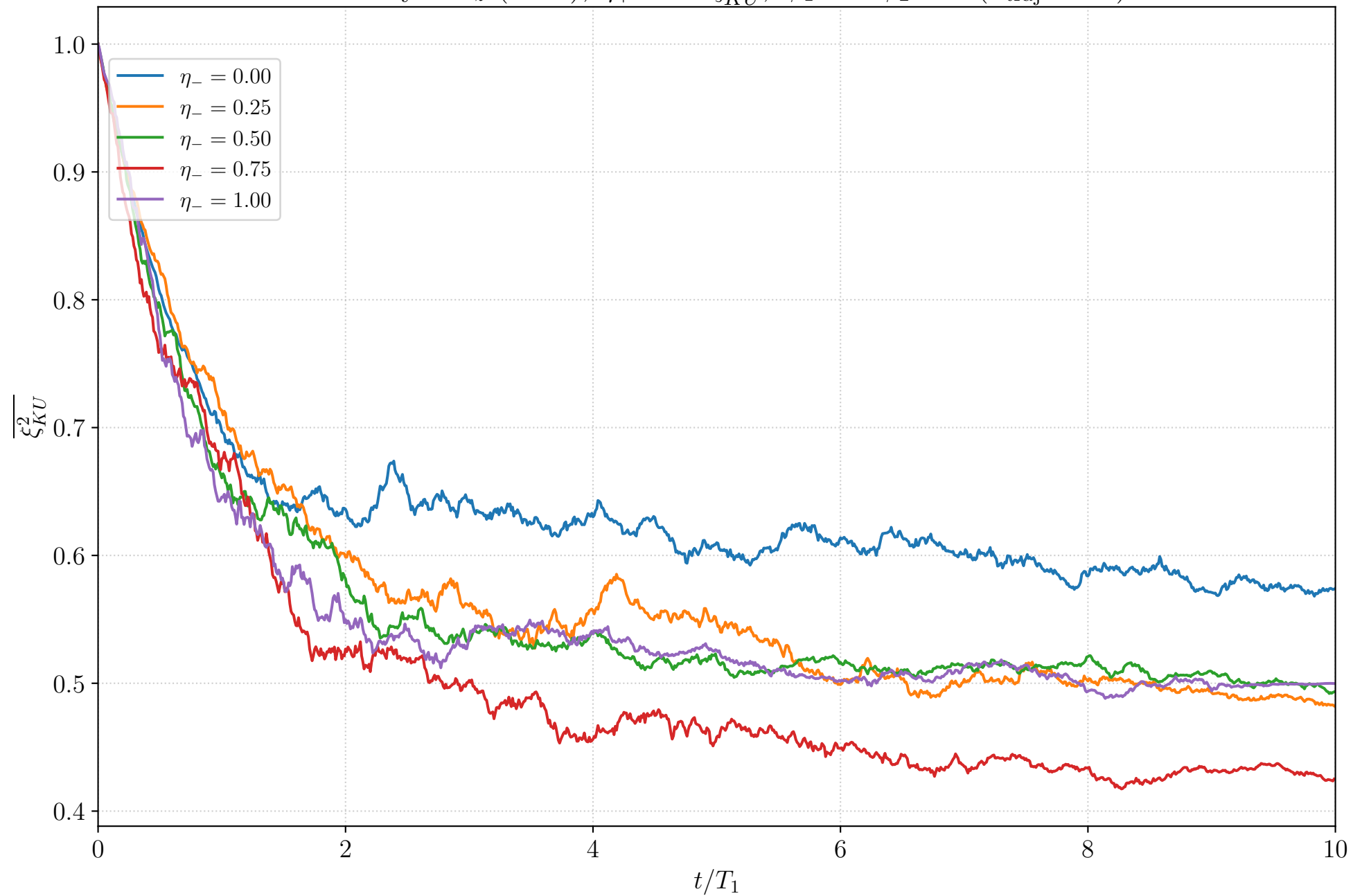
Homodyne J_z (N=2), \eta_+ = 1 : \overline{\xi_{KU}^2} , \phi_1 = 0 \phi_2 = 0 ( n_{\text{traj}} = 50 )
