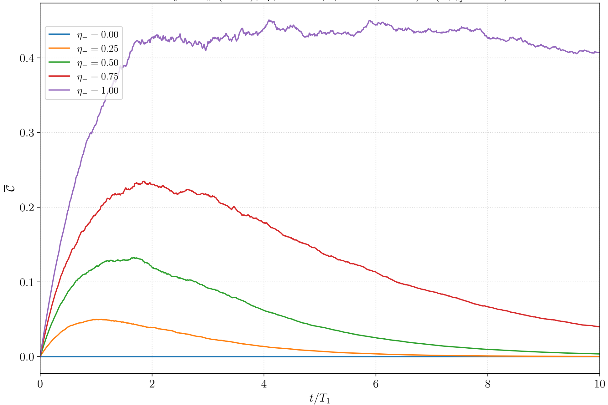
Homodyne J_z ( N=2 ), \eta_+ = 1 : \overline{\mathcal{C}} , \phi_1 = 0 \phi_2 = \pi/2 ( n_{\text{traj}} = 100 )
