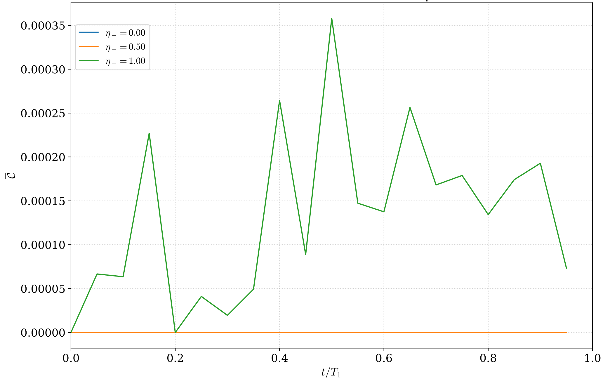
Homodyne J_z ( N=2 ), \eta_+ = 1 : \bar{\mathcal{C}} ( n_{\text{traj}}=10 )
