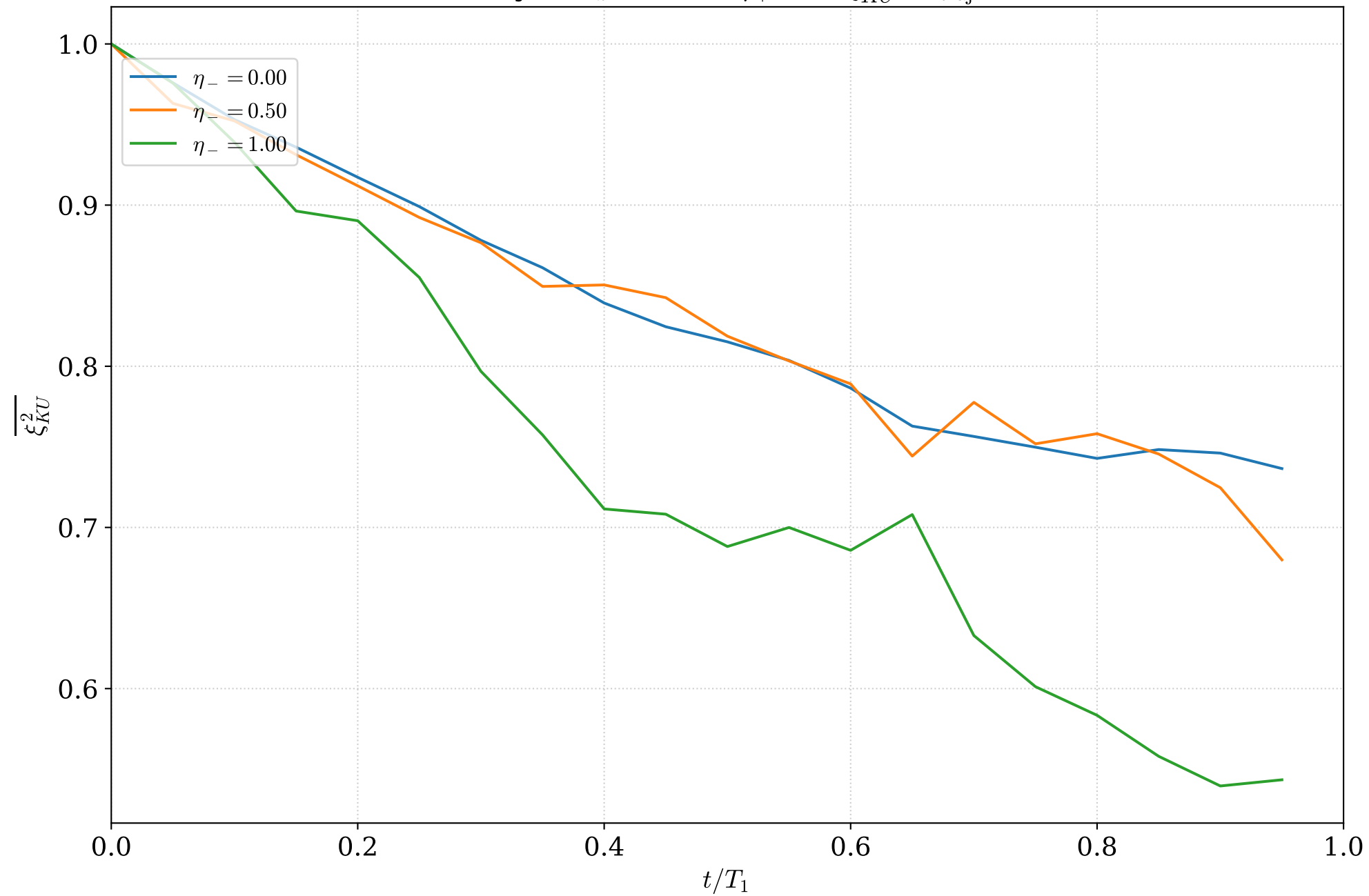
Homodyne J_z ( N=2 ), \eta_+ = 1 : \overline{\xi_{KU}^2} ( n_{\text{traj}}=10 )
