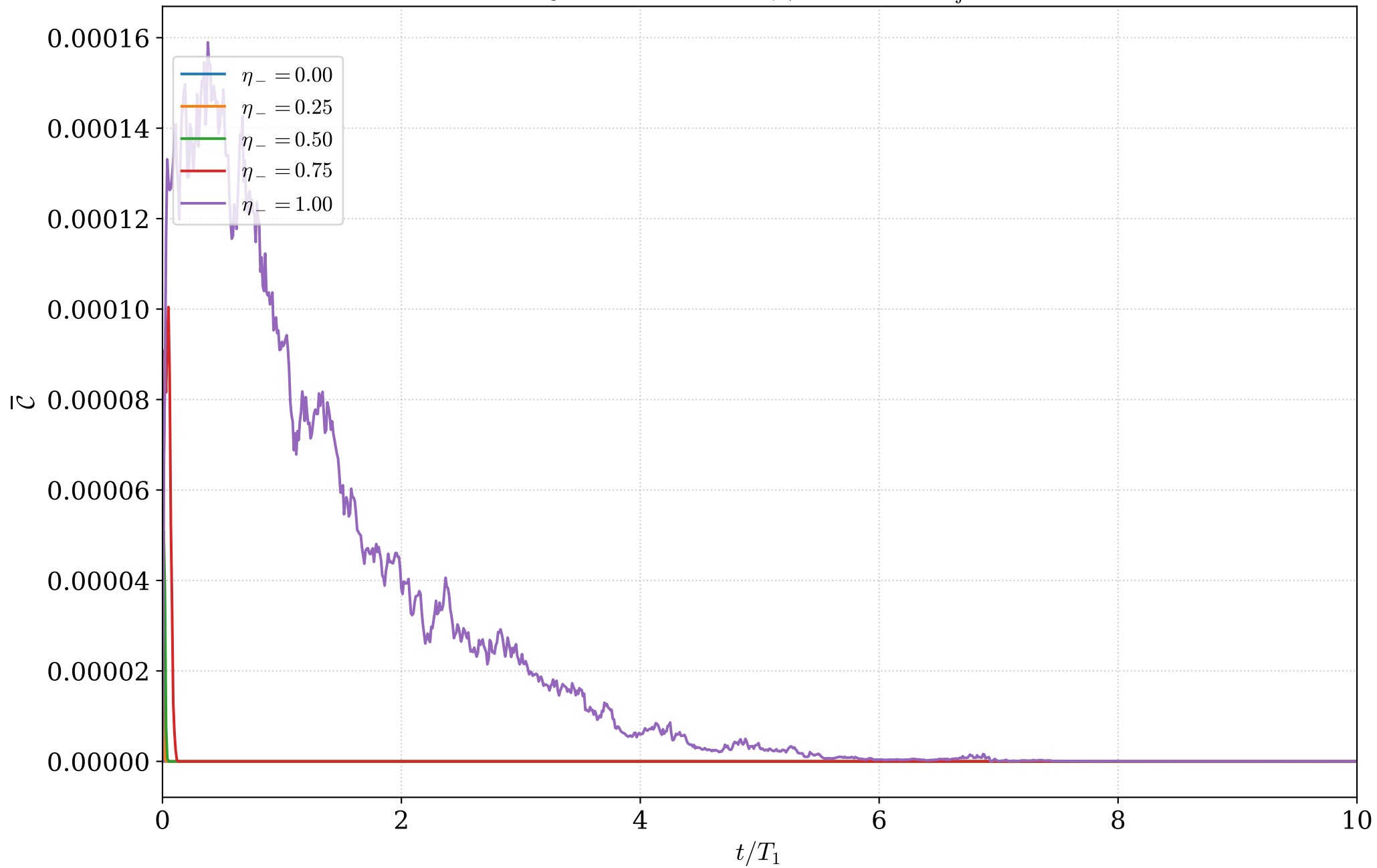
Homodyne J_z ( N=2 ), \eta_+ = 1 : \bar{\mathcal{C}} ( n_{\text{traj}}=1000 )
