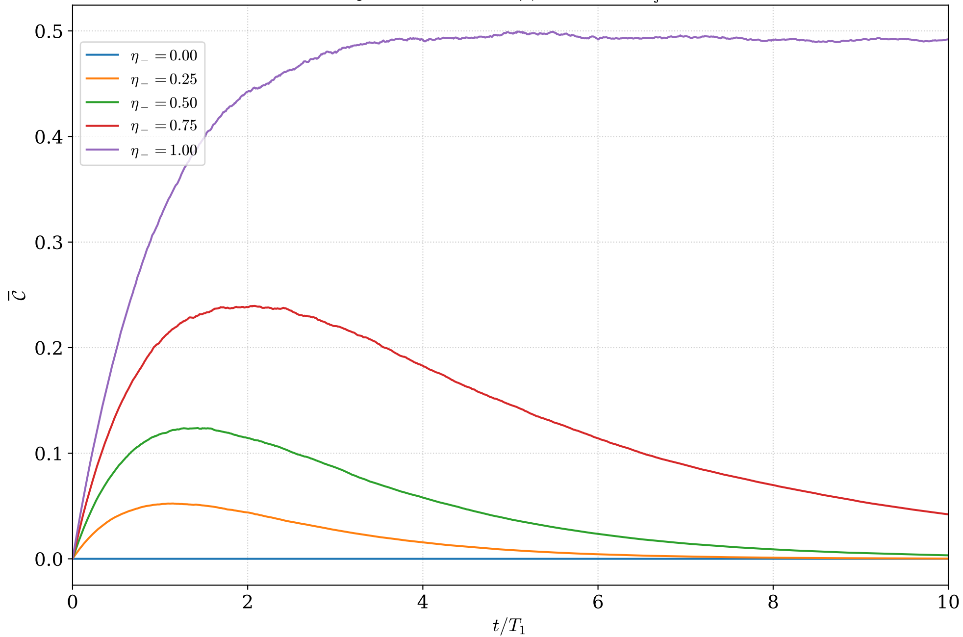
Homodyne J_z ( N=2 ), \eta_+ = 1 : \bar{c} ( n_{\text{traj}}=1000 )
