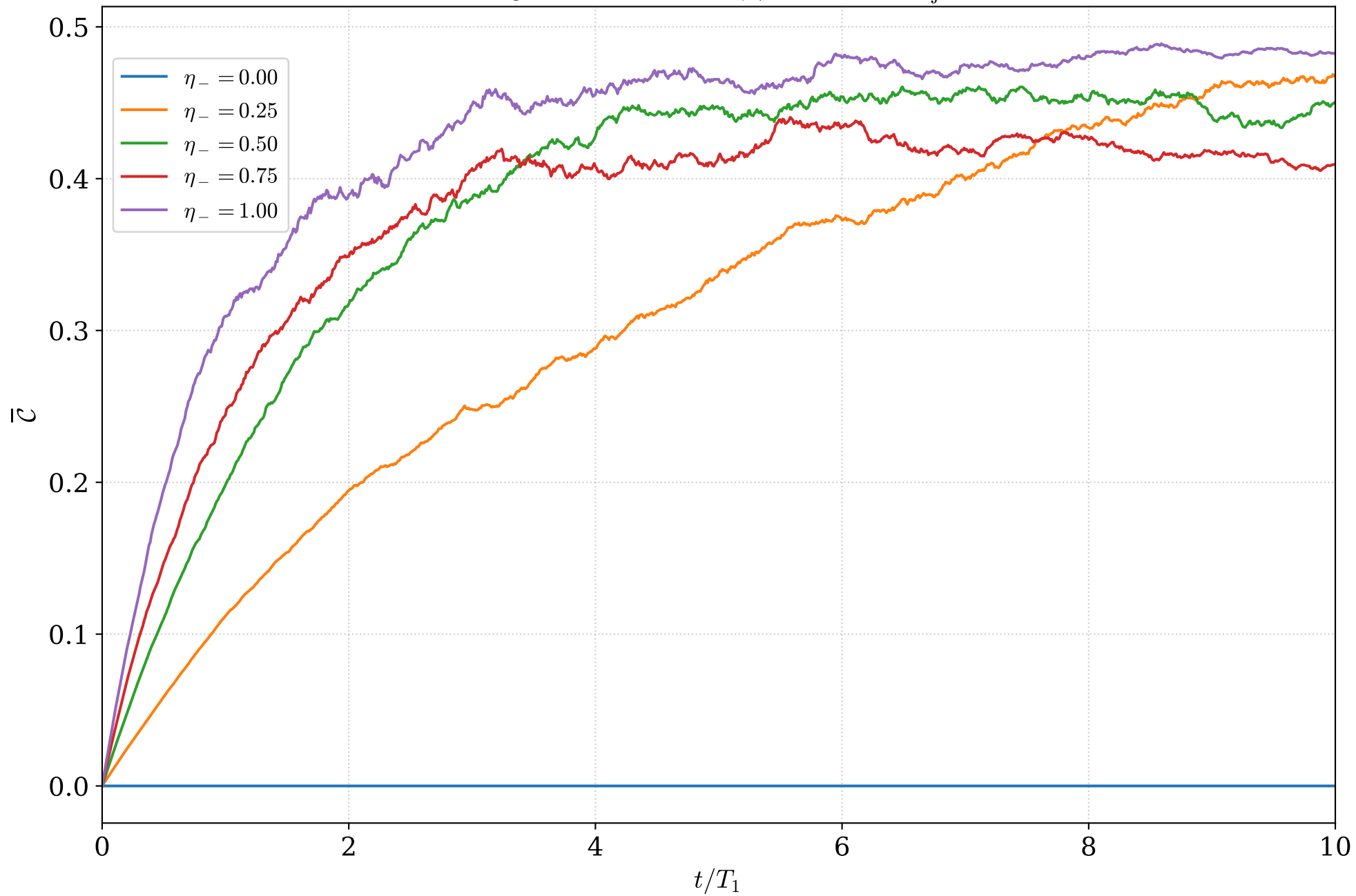
Homodyne J_z ( N=2 ), \eta_+ = 1 : \bar{\mathcal{C}} ( n_{\text{traj}}=100 )
