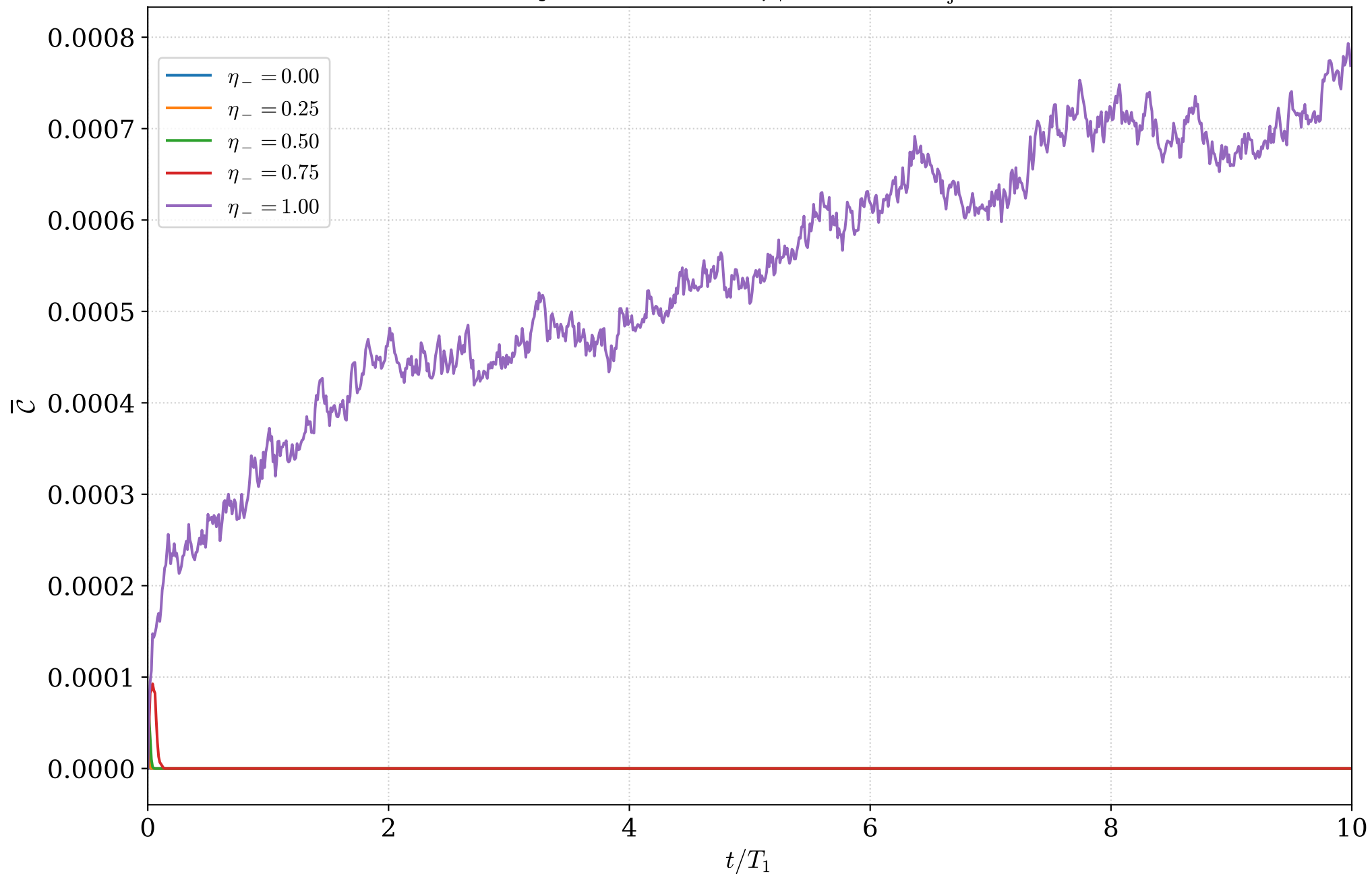
Homodyne J_z ( N=2 ), \eta_+ = 1 : \bar{C} ( n_{\text{traj}}=1000 )
