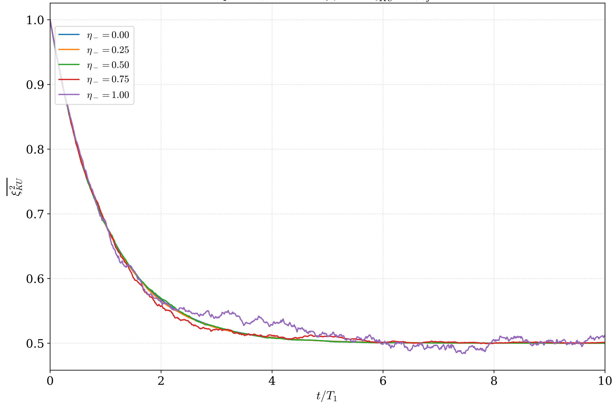
Homodyne J_z ( N=2 ), \eta_+ = 1 : \overline{\xi_{KU}^2} ( n_{\text{traj}}=1000 )
