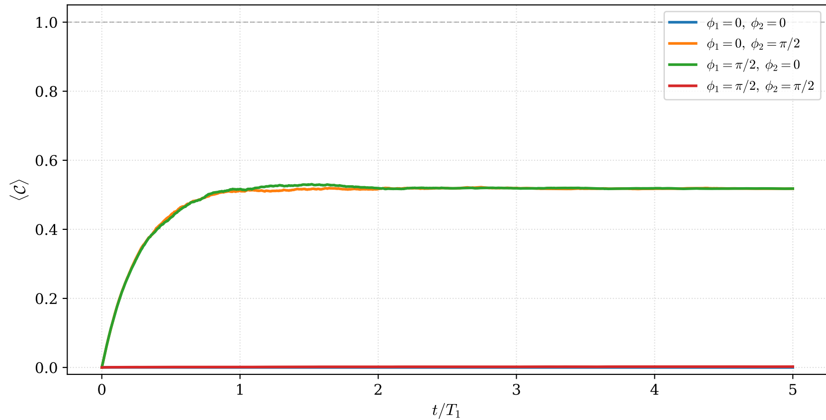
Ensemble-average concurrence — PlusPlus, \eta_1 = 1.0 , \eta_2 = 1.0 , ntraj = 1000
